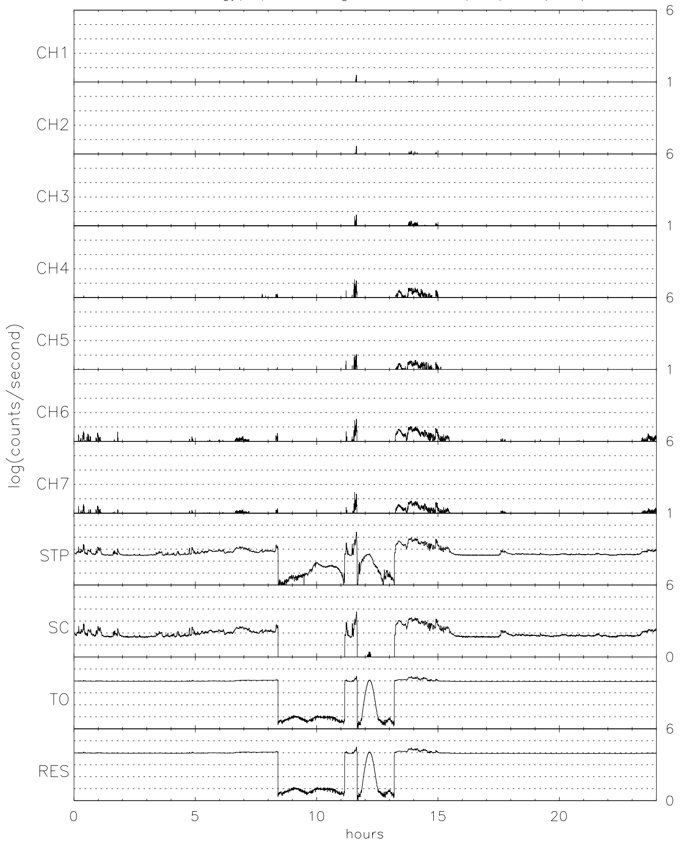
TIDE energy/spin averaged H+ for 06/18/96 (170)
