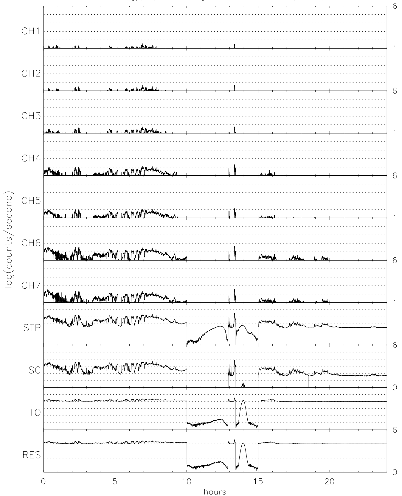
TIDE energy/spin averaged H+ for 06/15/96 (167)
