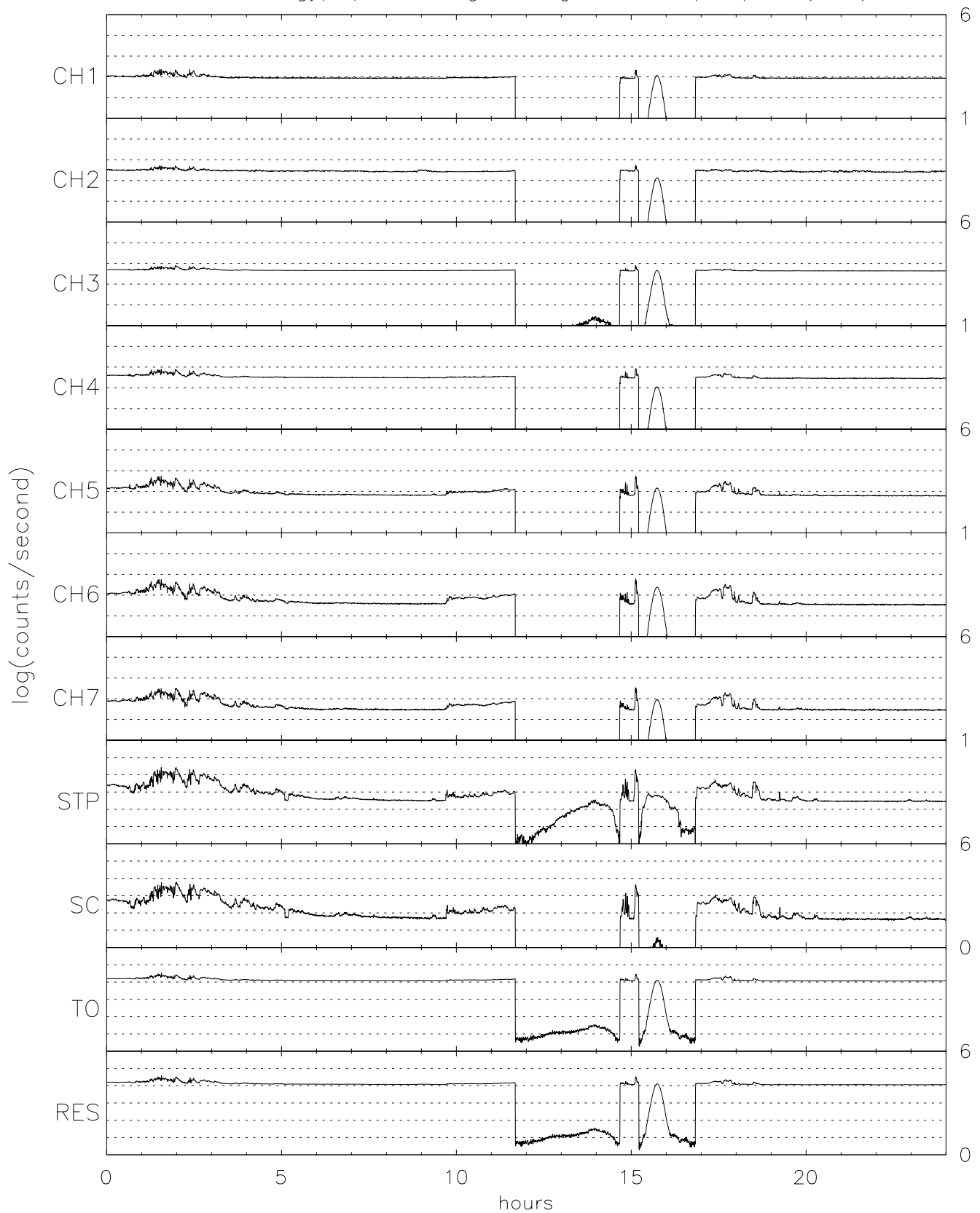
TIDE energy/spin averaged Singles for 06/12/96 (164)
