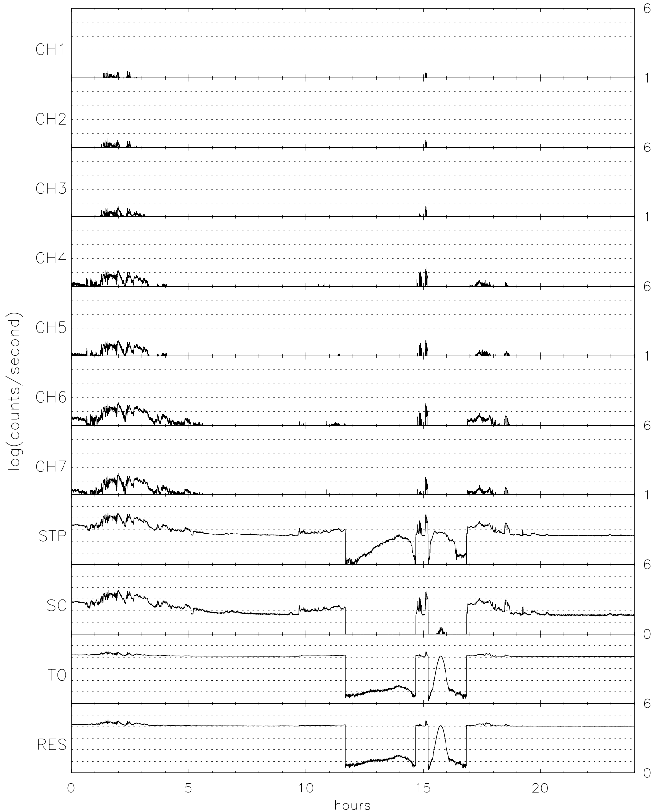
TIDE energy/spin averaged H+ for 06/12/96 (164)
