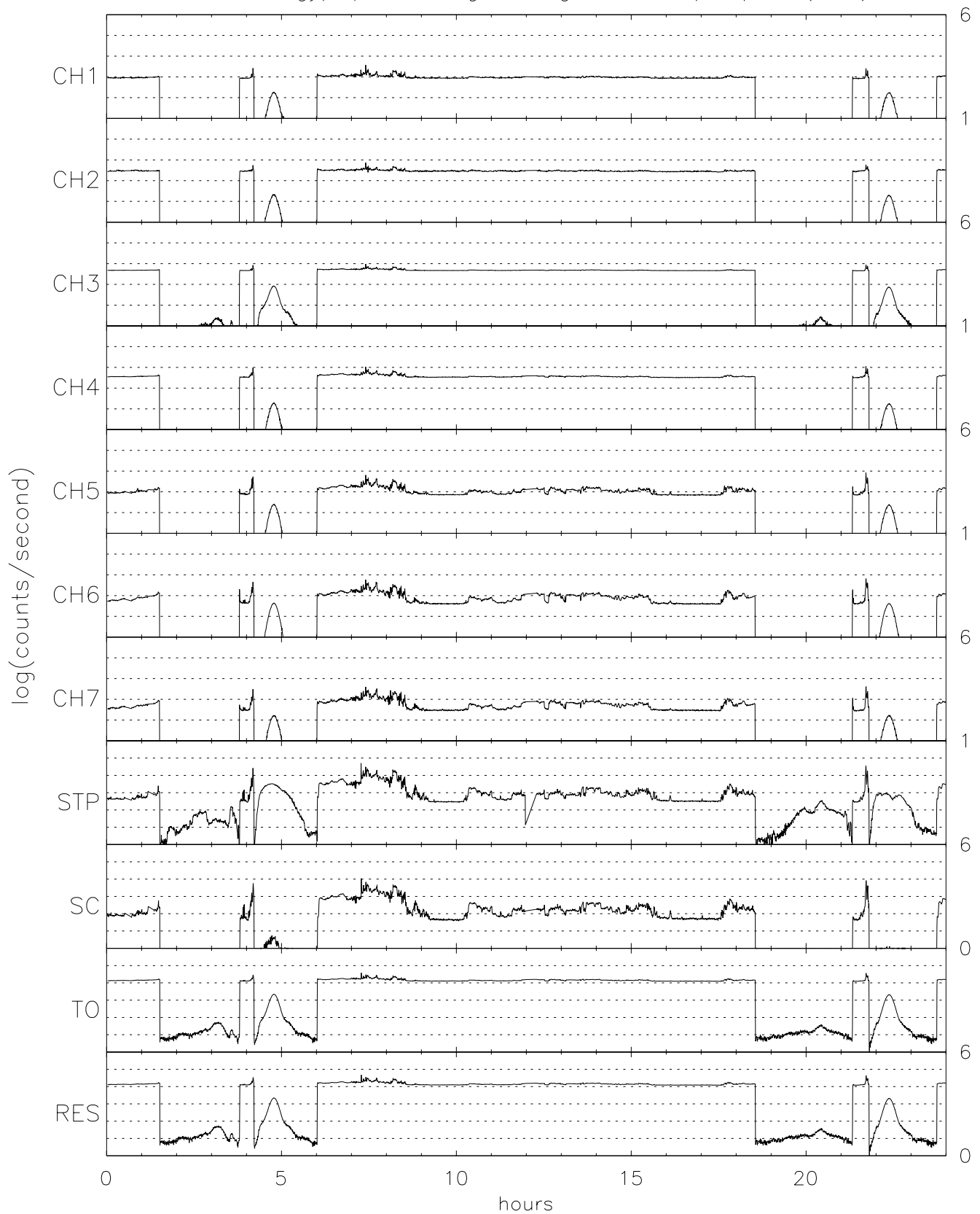
TIDE energy/spin averaged Singles for 06/11/96 (163)
