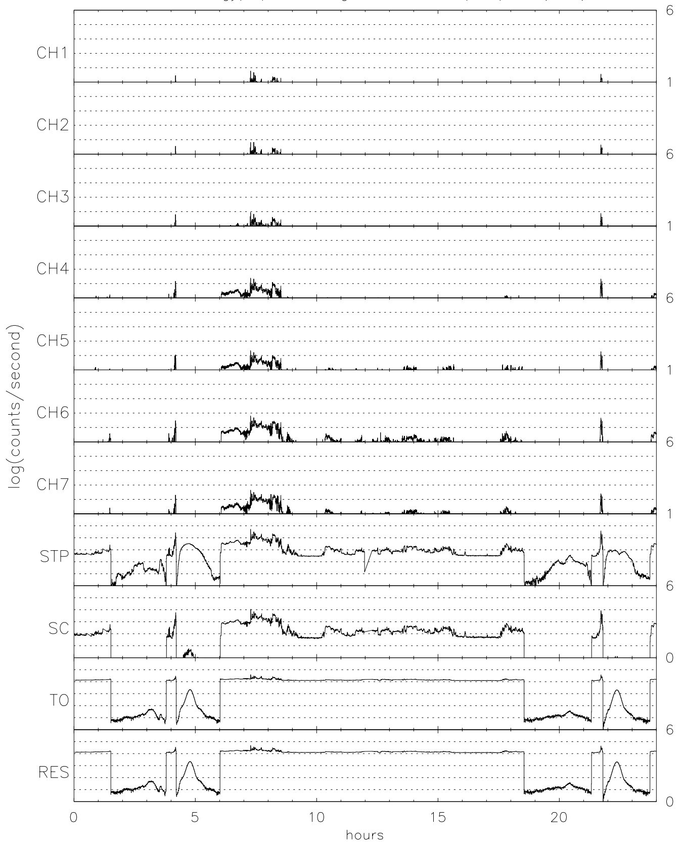
TIDE energy/spin averaged H+ for 06/11/96 (163)
