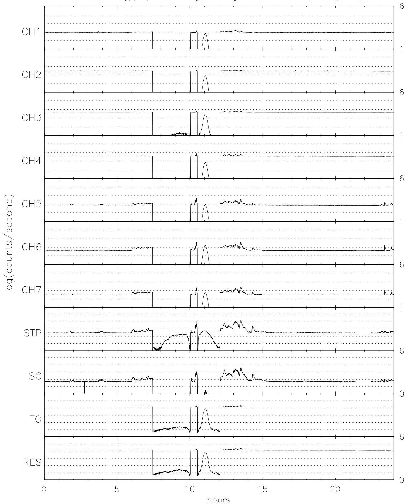
TIDE energy/spin averaged Singles for 06/10/96 (162)
