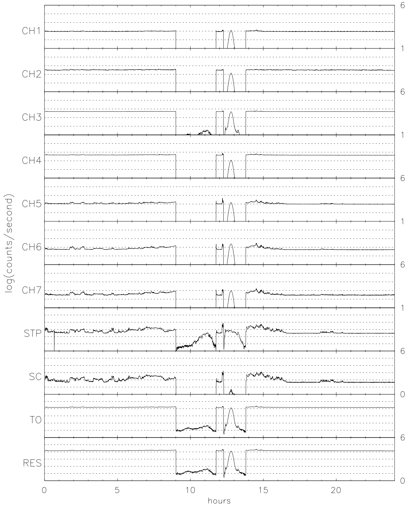
TIDE energy/spin averaged Singles for 06/07/96 (159)
