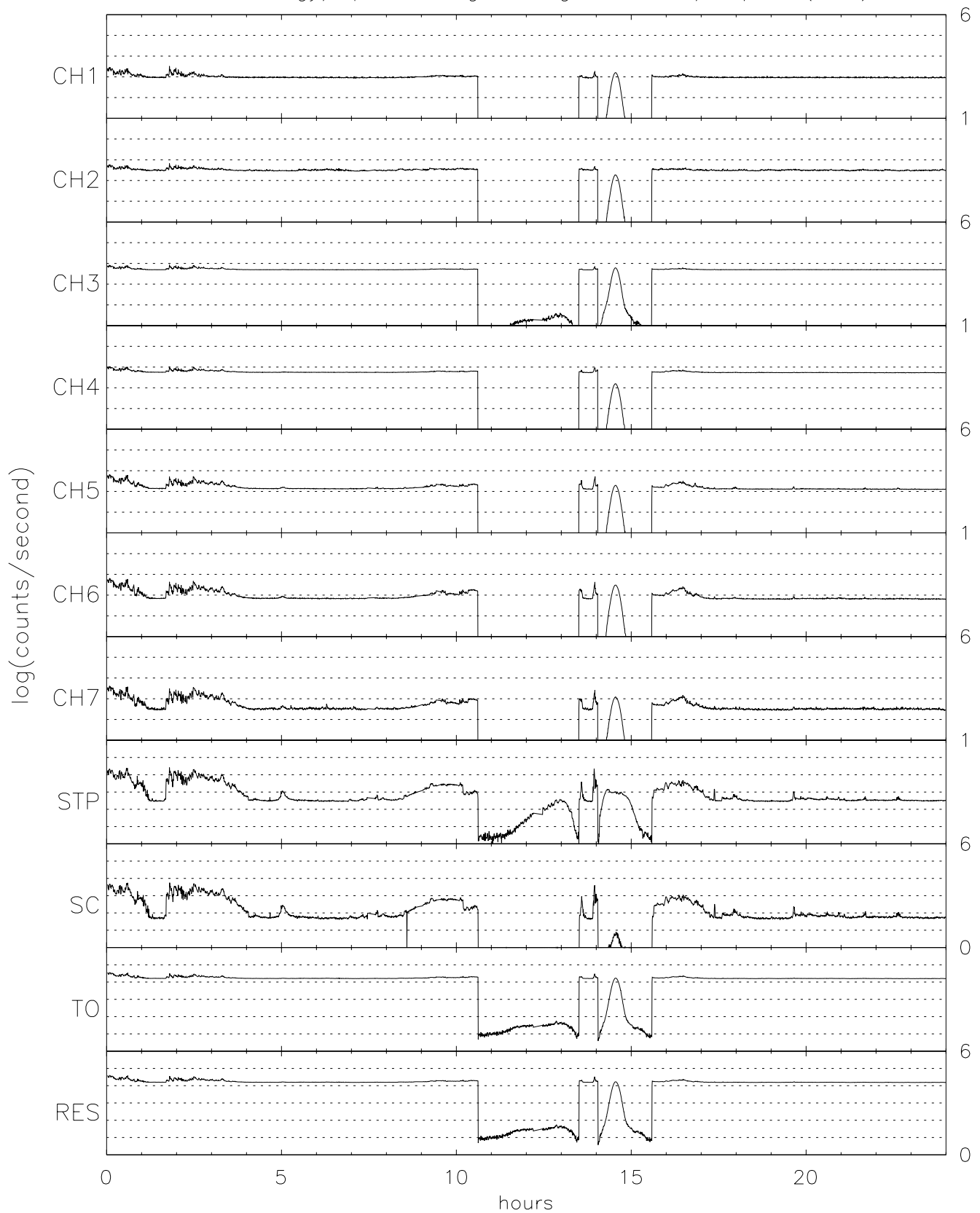
TIDE energy/spin averaged Singles for 06/04/96 (156)
