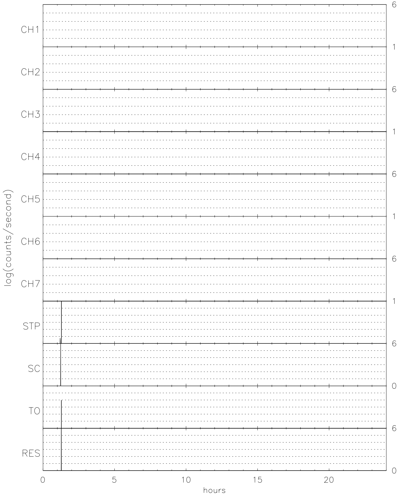
TIDE energy/spin averaged Singles for 06/01/96 (153)
