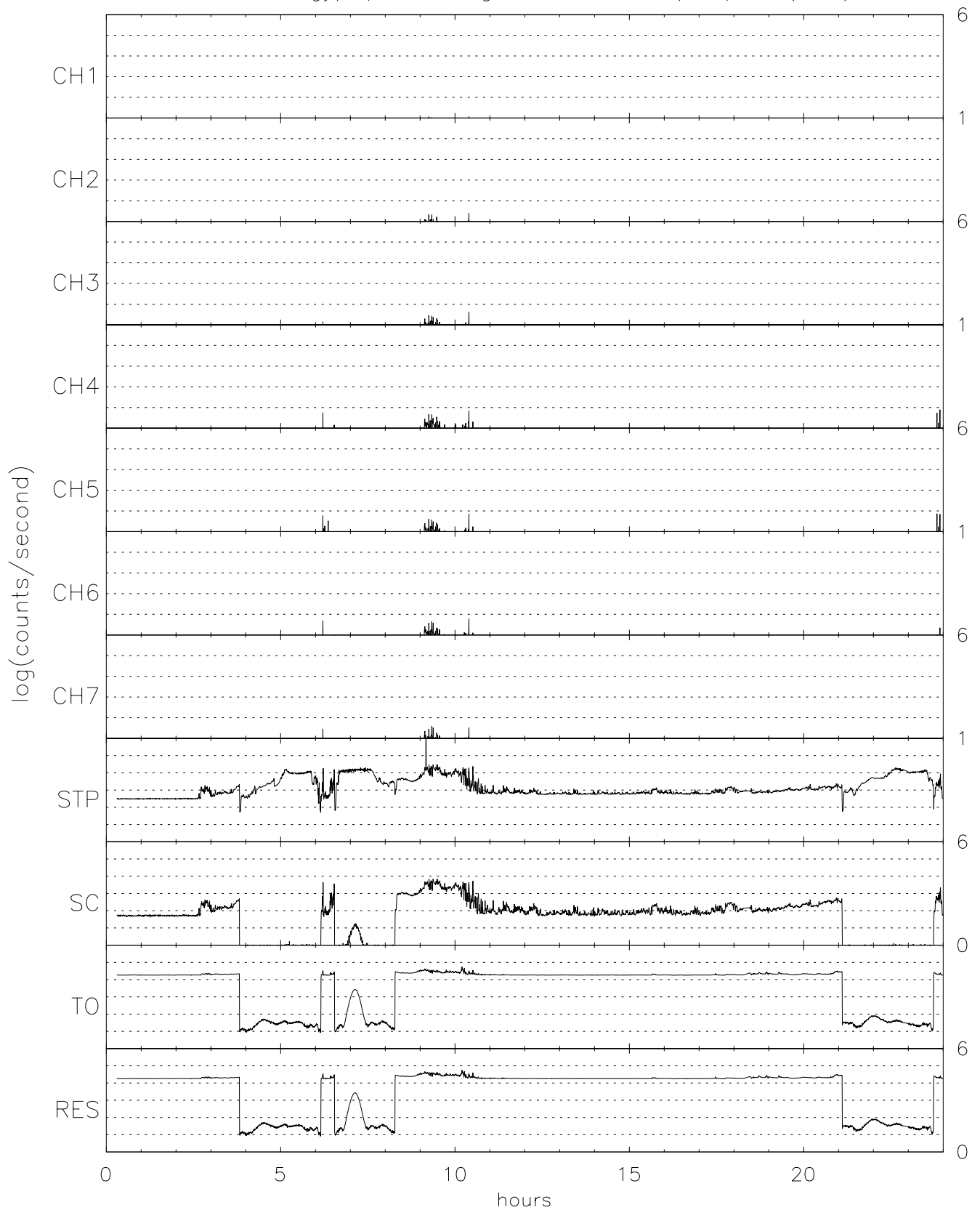
TIDE energy/spin averaged NO+ for 05/28/96 (149)
