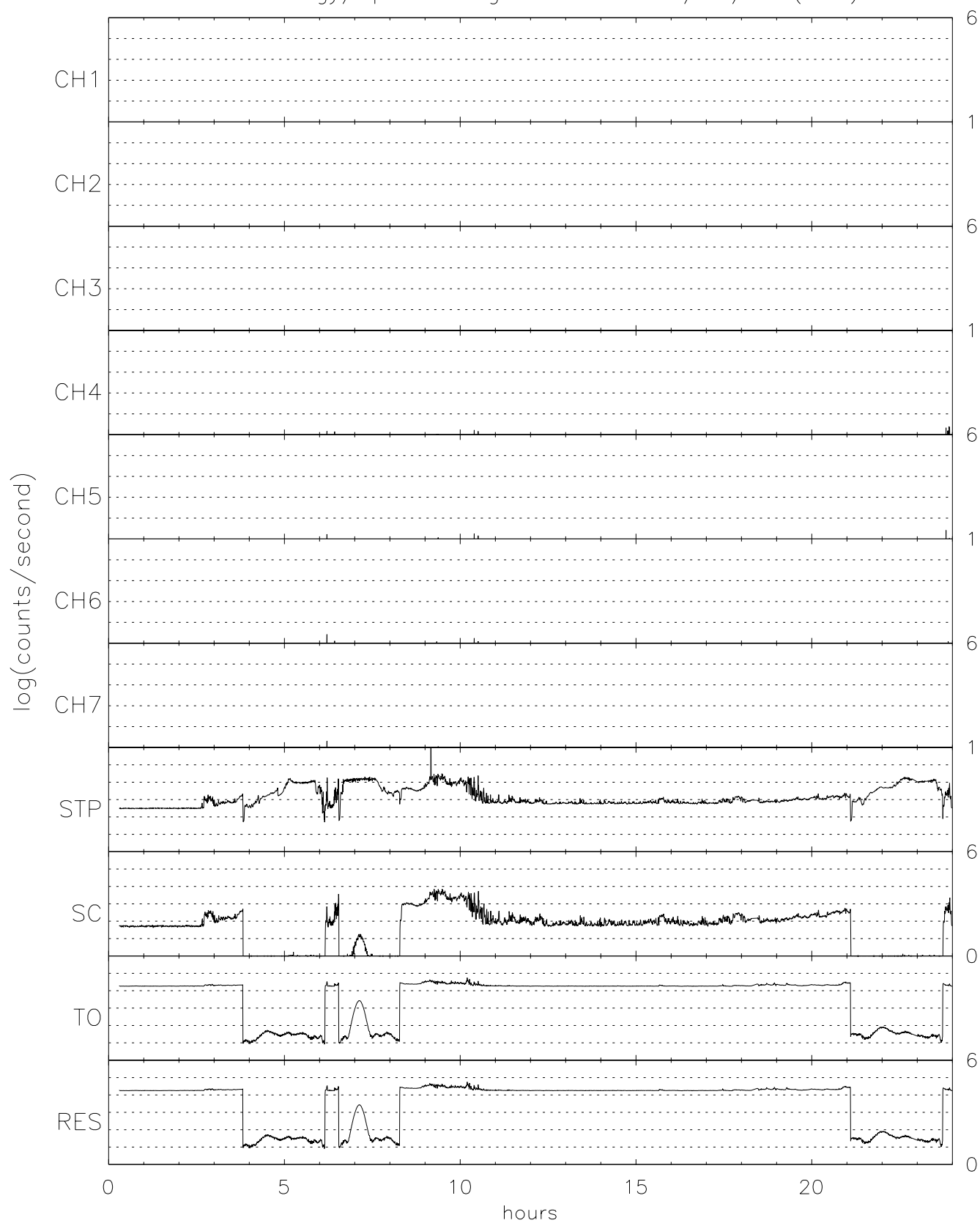
TIDE energy/spin averaged He+ for 05/28/96 (149)
