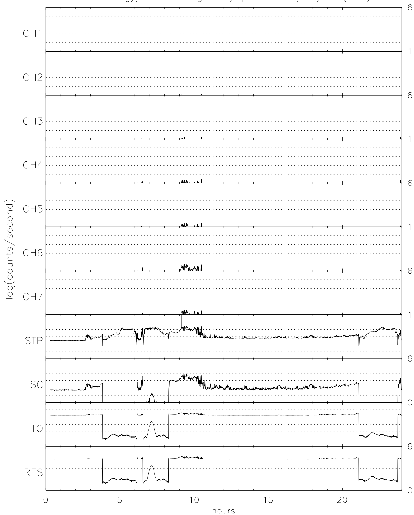
TIDE energy/spin averaged m/q=2 for 05/28/96 (149)
