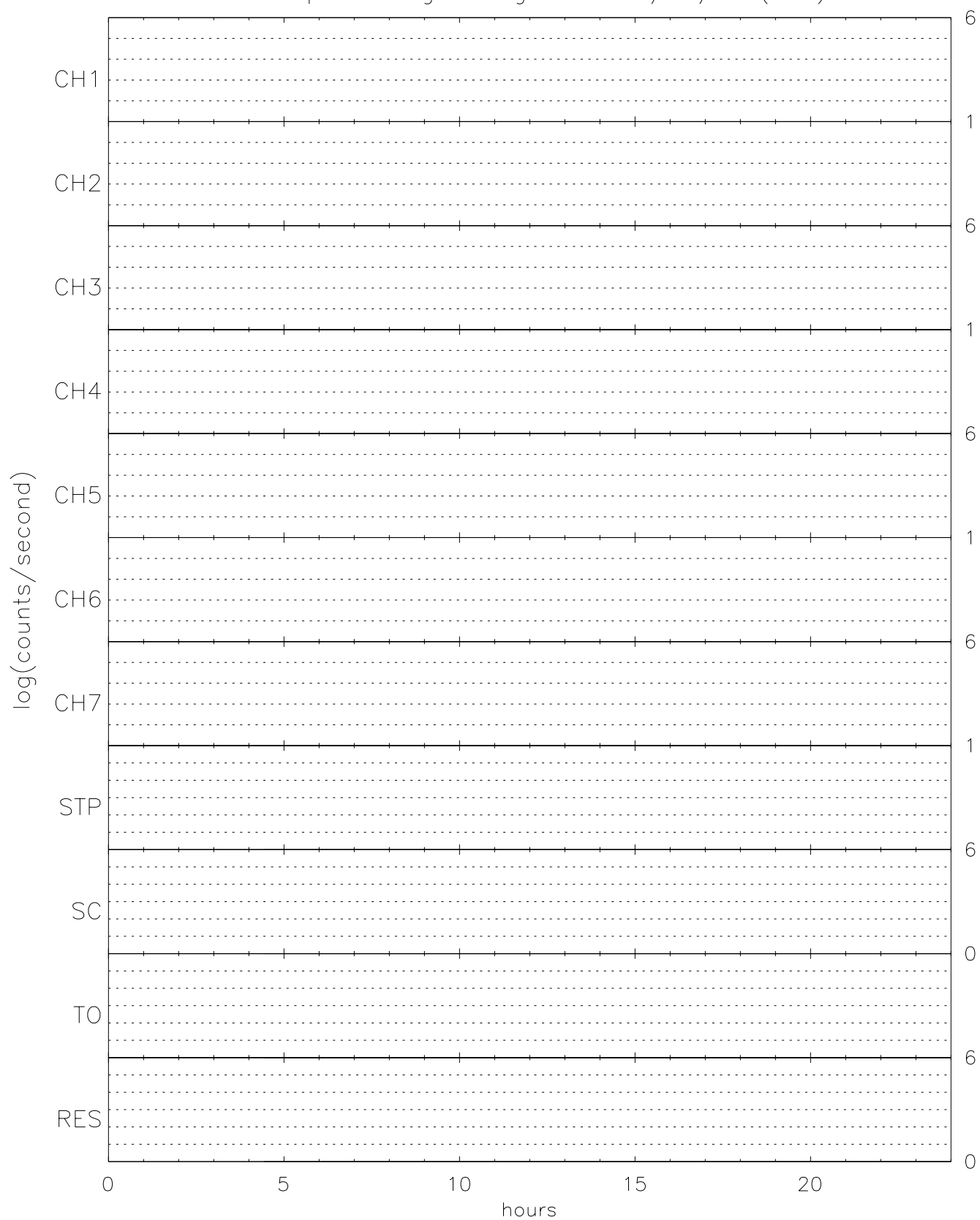
TIDE spin averaged Singles for 05/25/96 (146)
