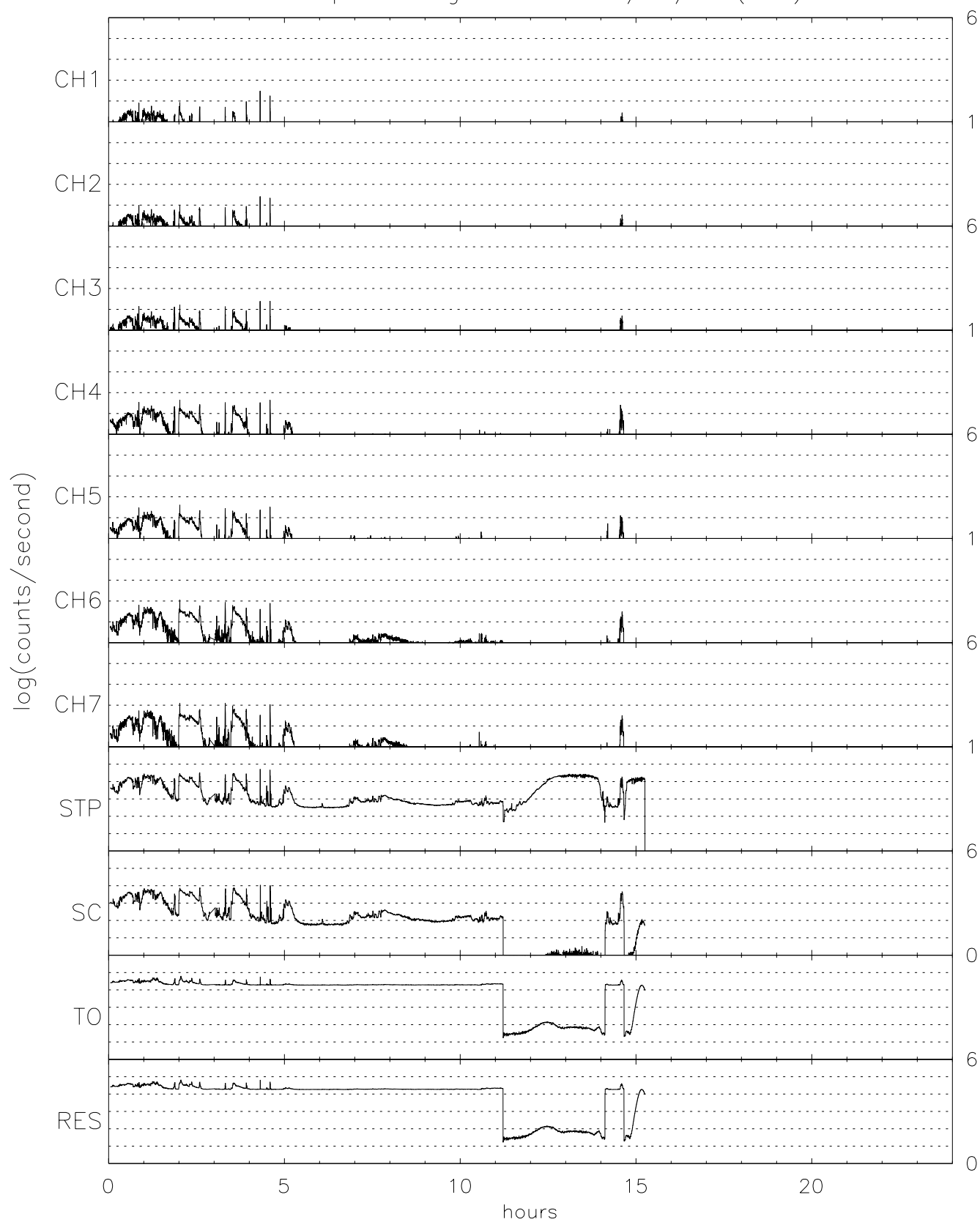
TIDE spin averaged h+ for 05/24/96 (145)
