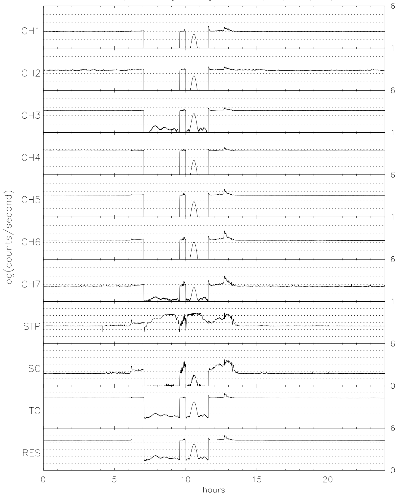
TIDE spin averaged Singles for 05/22/96 (143)
