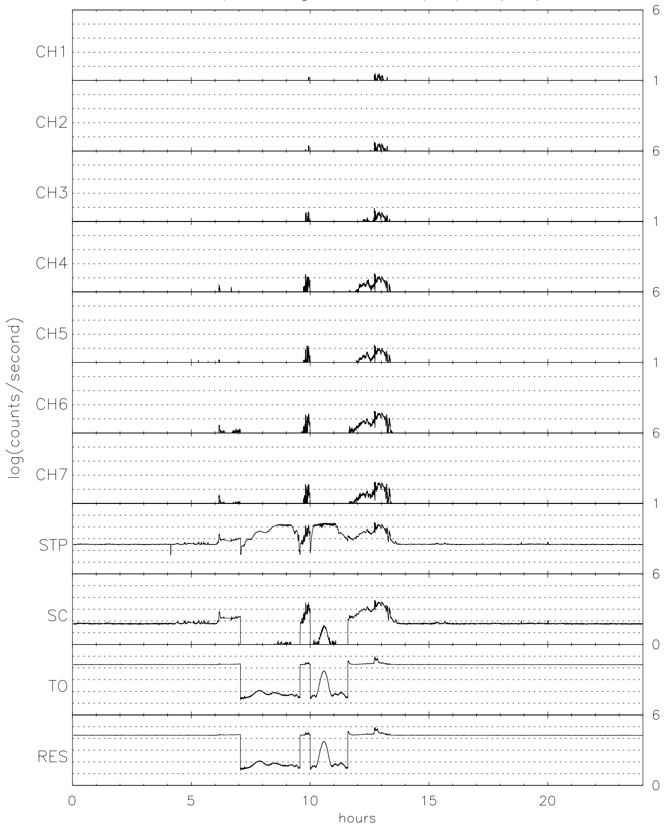
TIDE spin averaged H+ for 05/22/96 (143)
