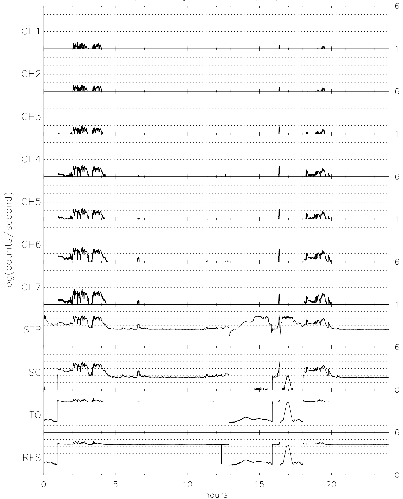
TIDE spin averaged H+ for 05/21/96 (142)
