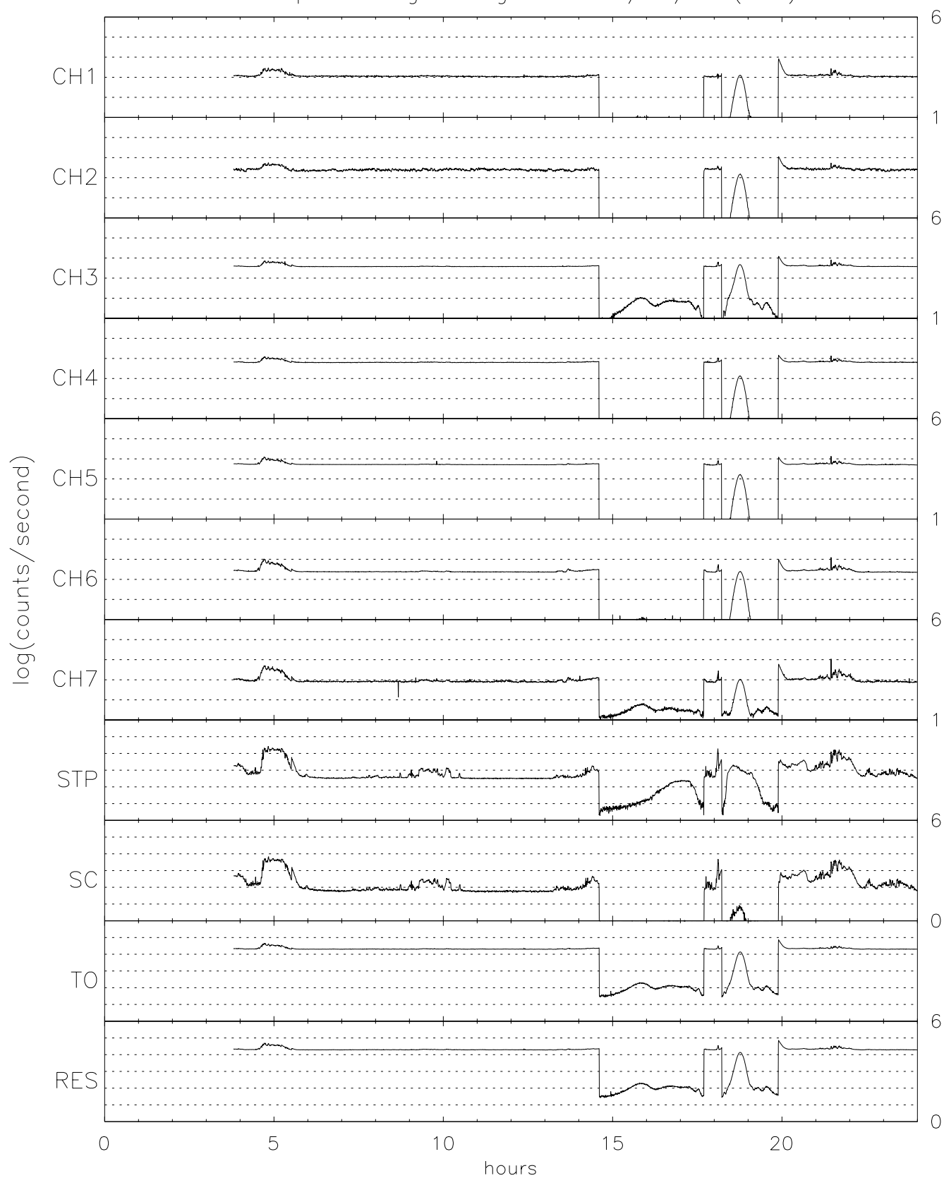
TIDE spin averaged Singles for 05/18/96 (139)
