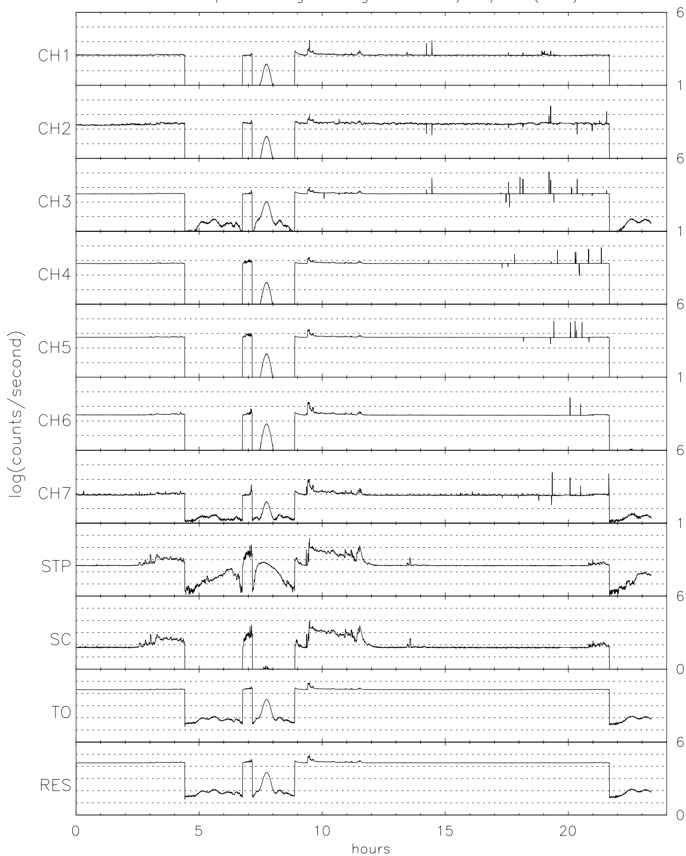
TIDE spin averaged Singles for 05/17/96 (138)
