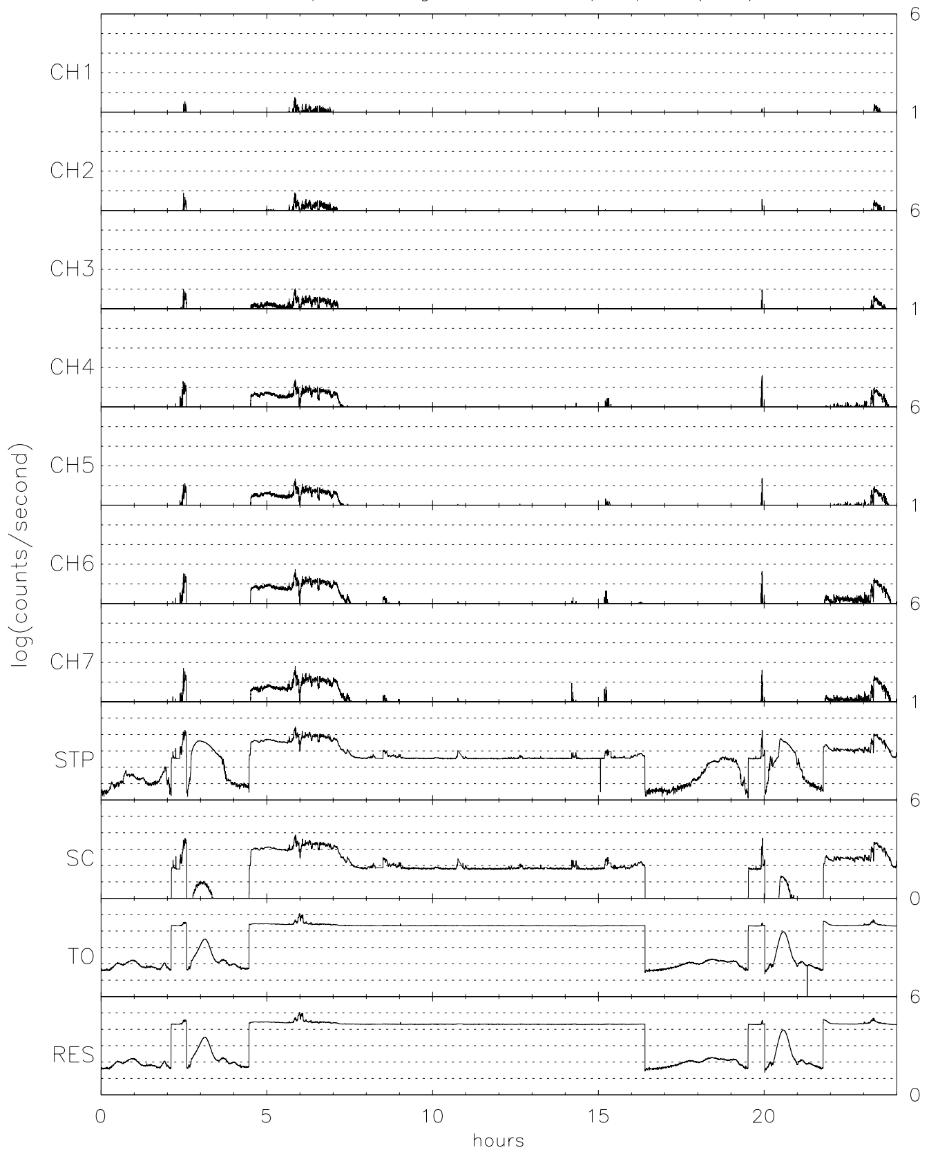
TIDE spin averaged H+ for 05/15/96 (136)
