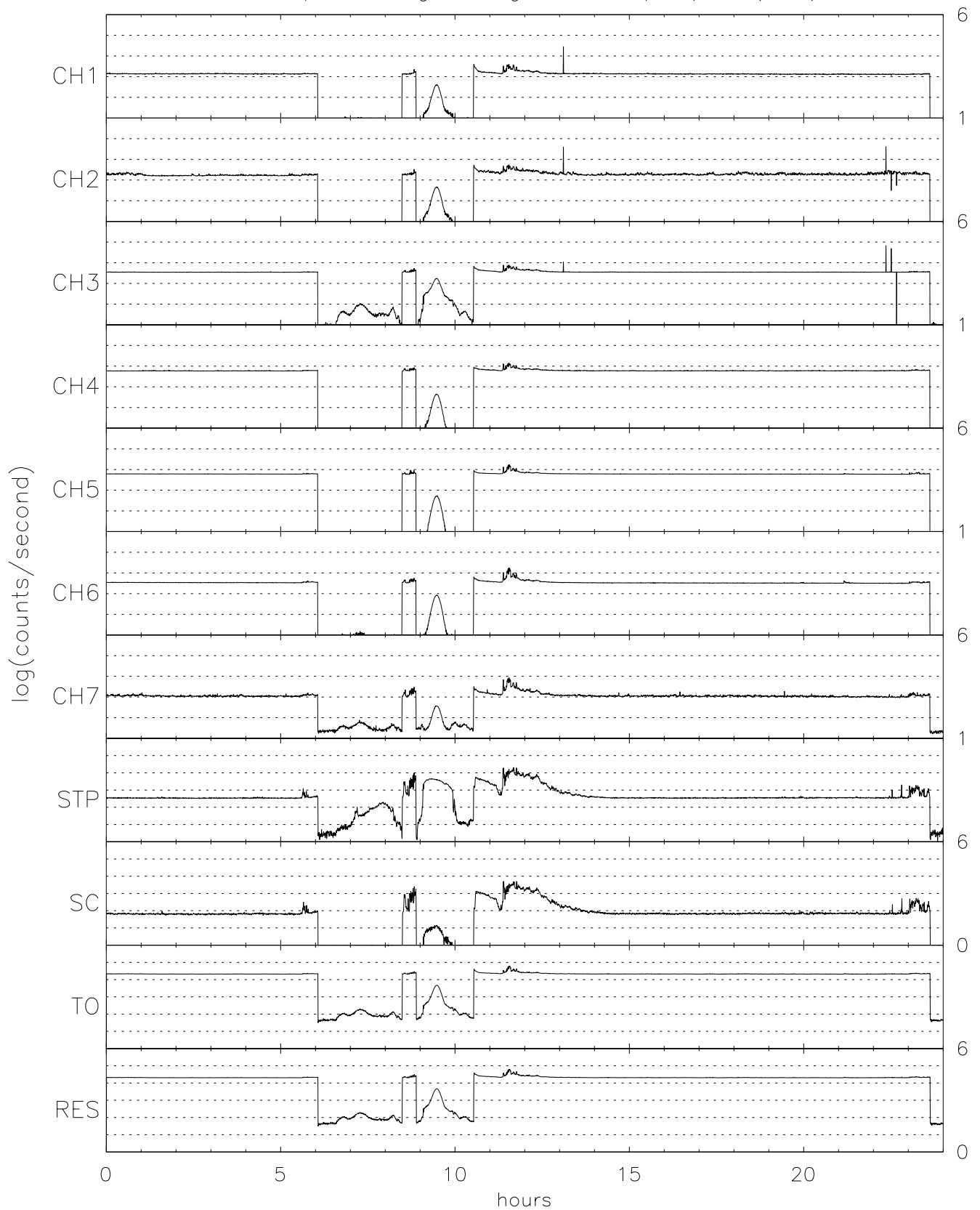
TIDE spin averaged Singles for 05/14/96 (135)
