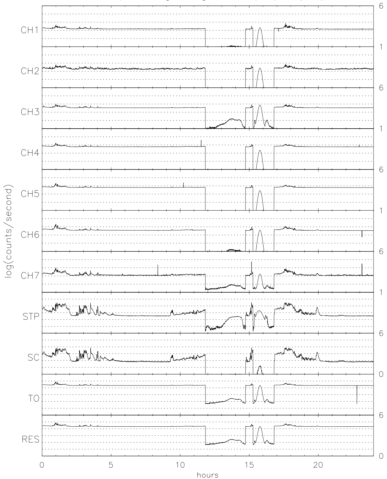
TIDE spin averaged Singles for 05/13/96 (134)
