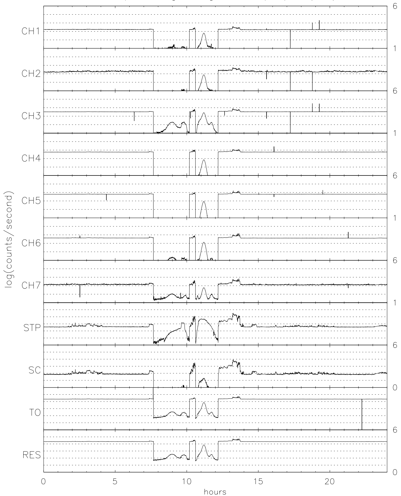
TIDE spin averaged Singles for 05/11/96 (132)
