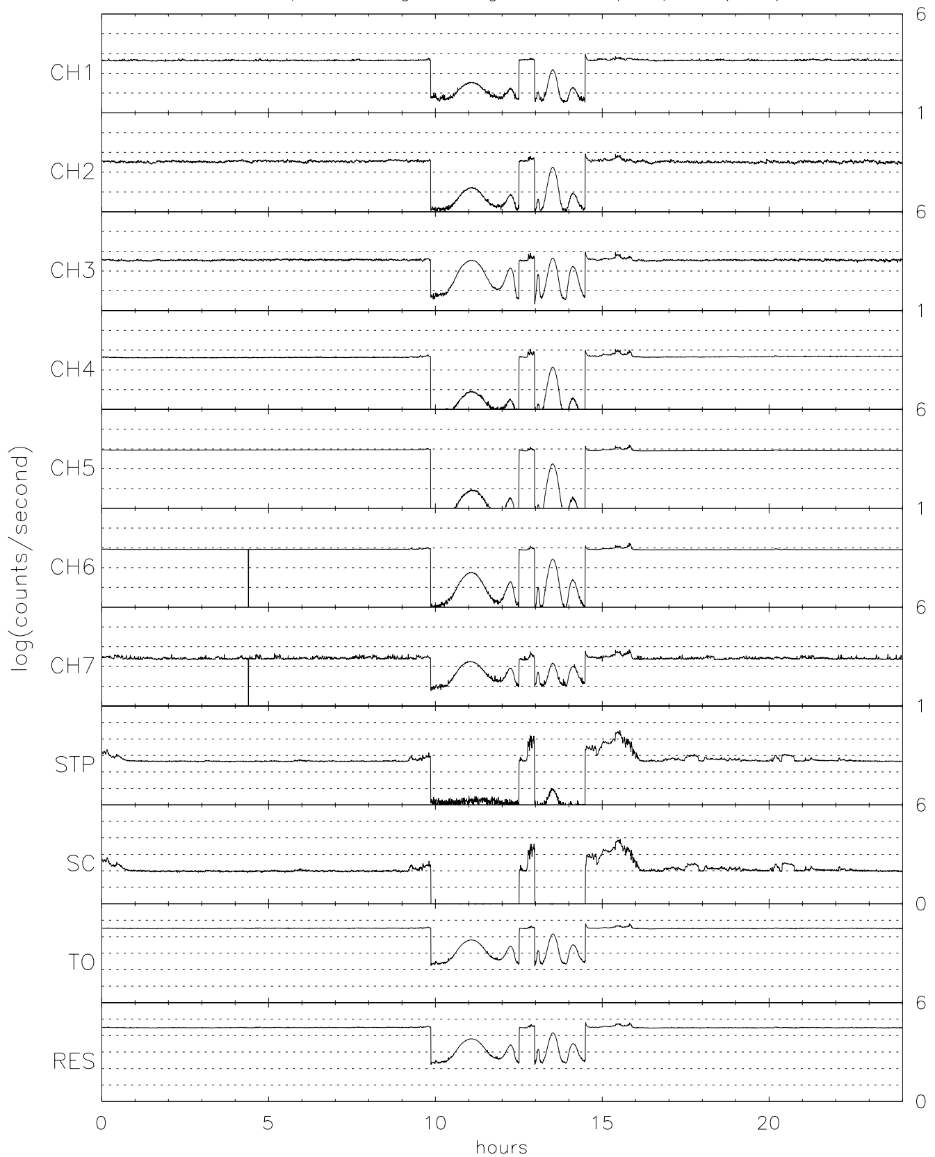
TIDE spin averaged Singles for 04/27/96 (118)
