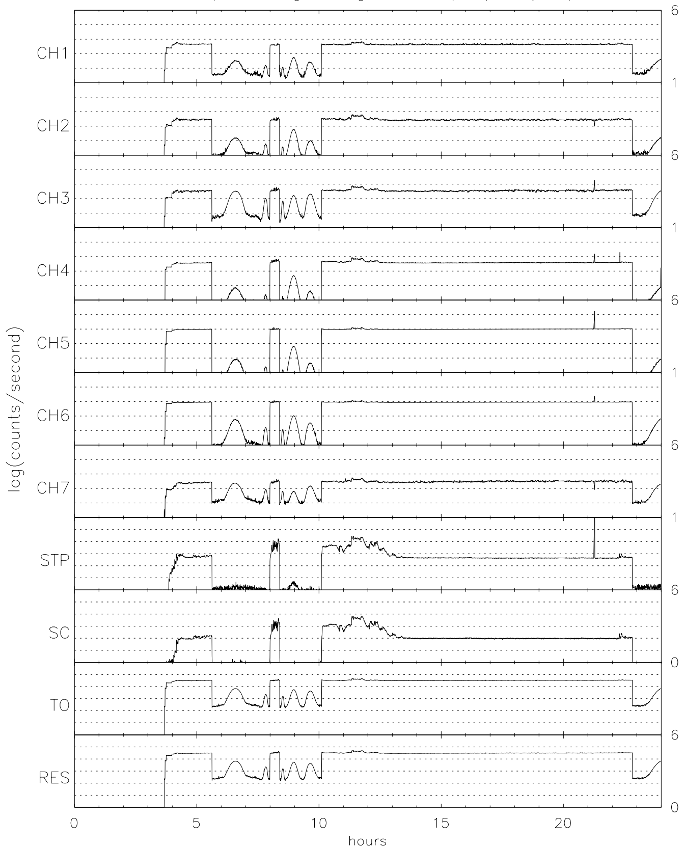
TIDE spin averaged Singles for 04/25/96 (116)
