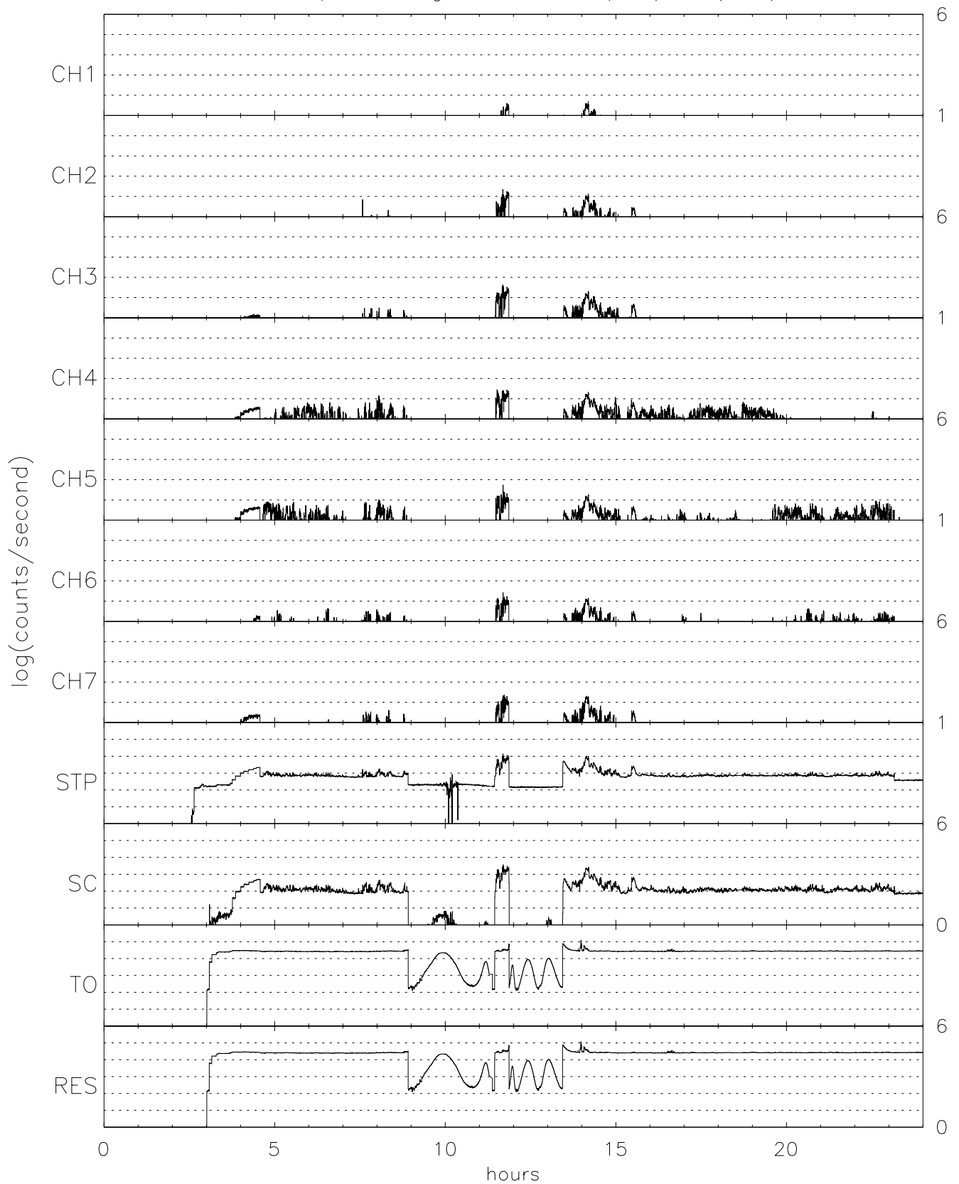
TIDE spin averaged H+ for 04/19/96 (110)
