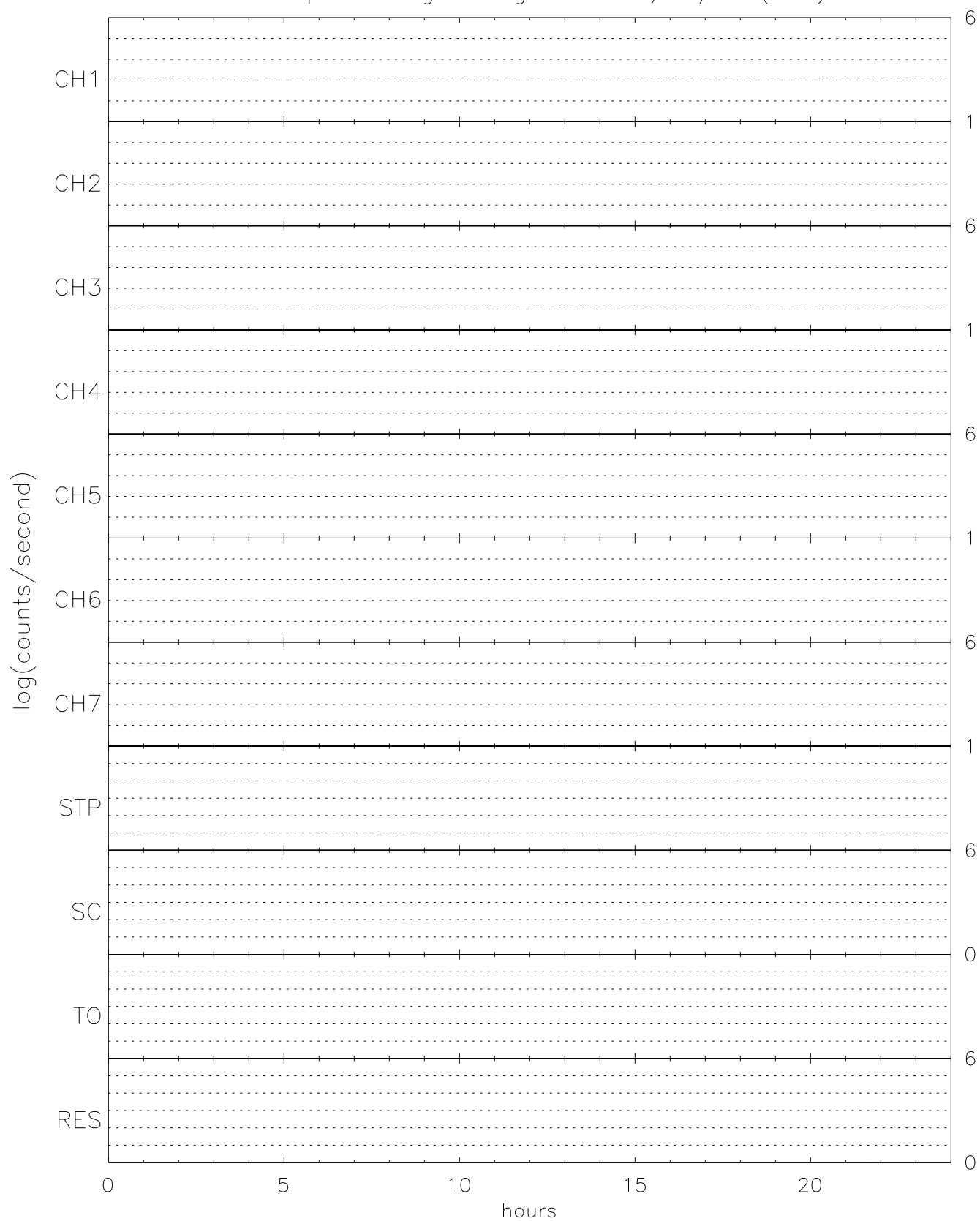
TIDE spin averaged Singles for 04/18/96 (109)
