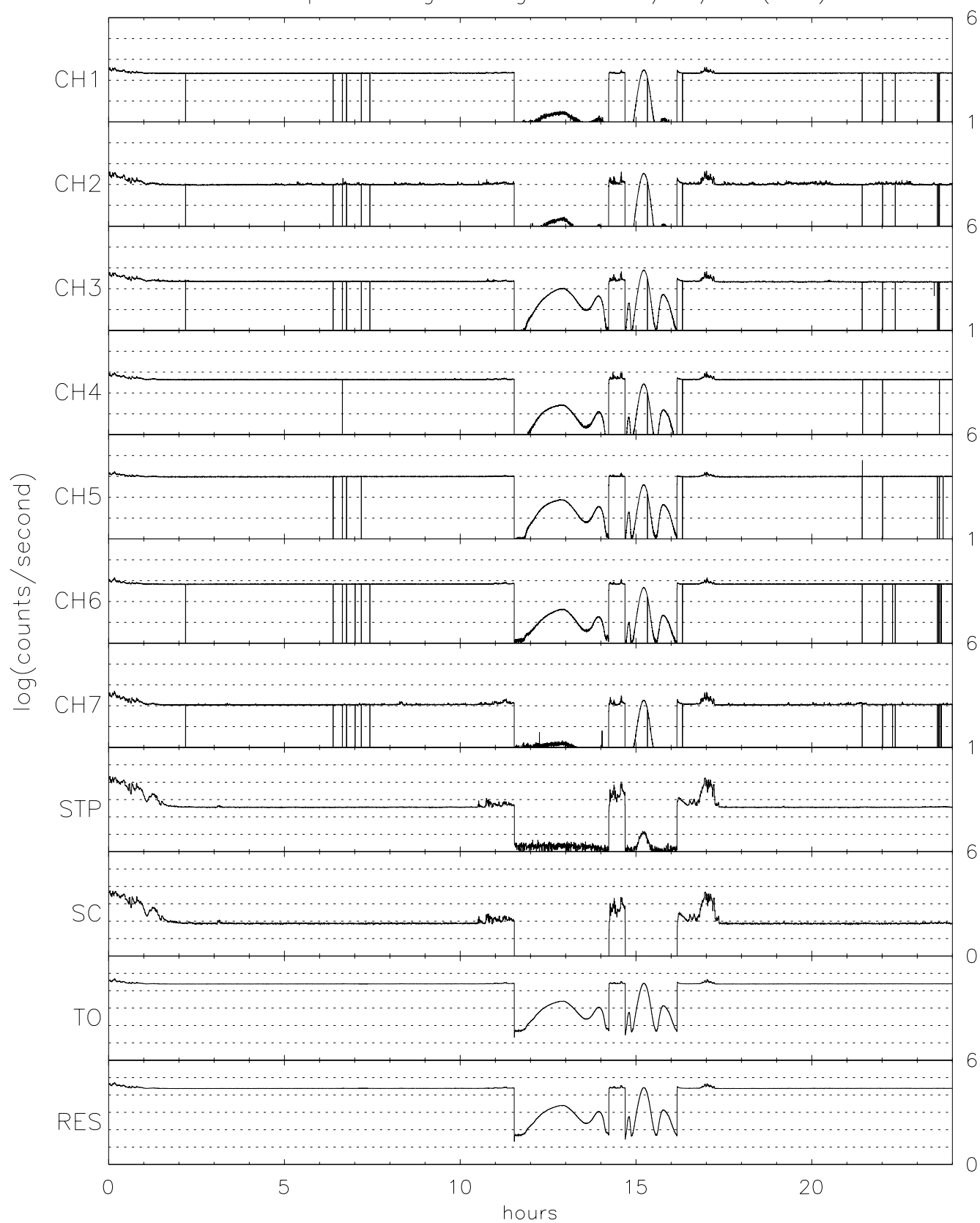
TIDE spin averaged Singles for 04/05/96 (096)
