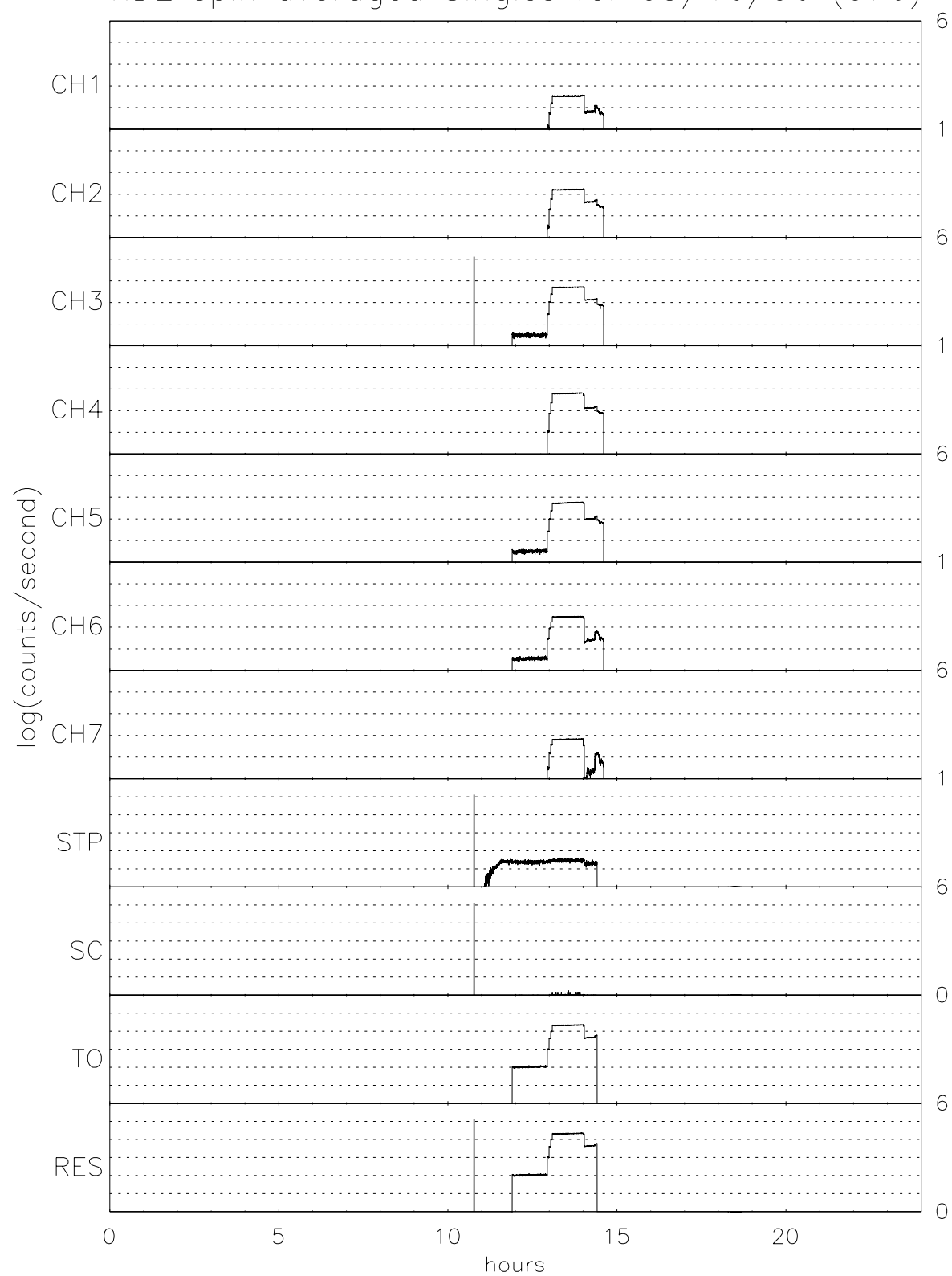
TIDE spin averaged Singles for 03/16/96 (076)
