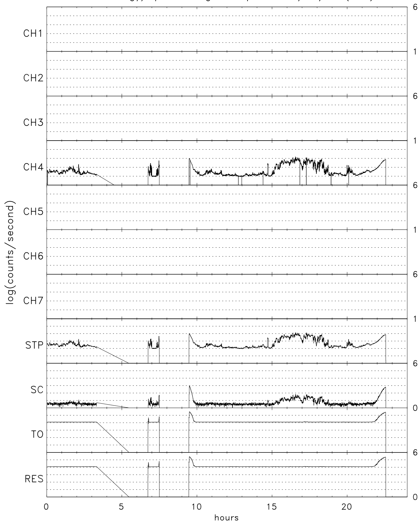
TIDE energy/spin averaged Stops for 01/10/08 (010)
