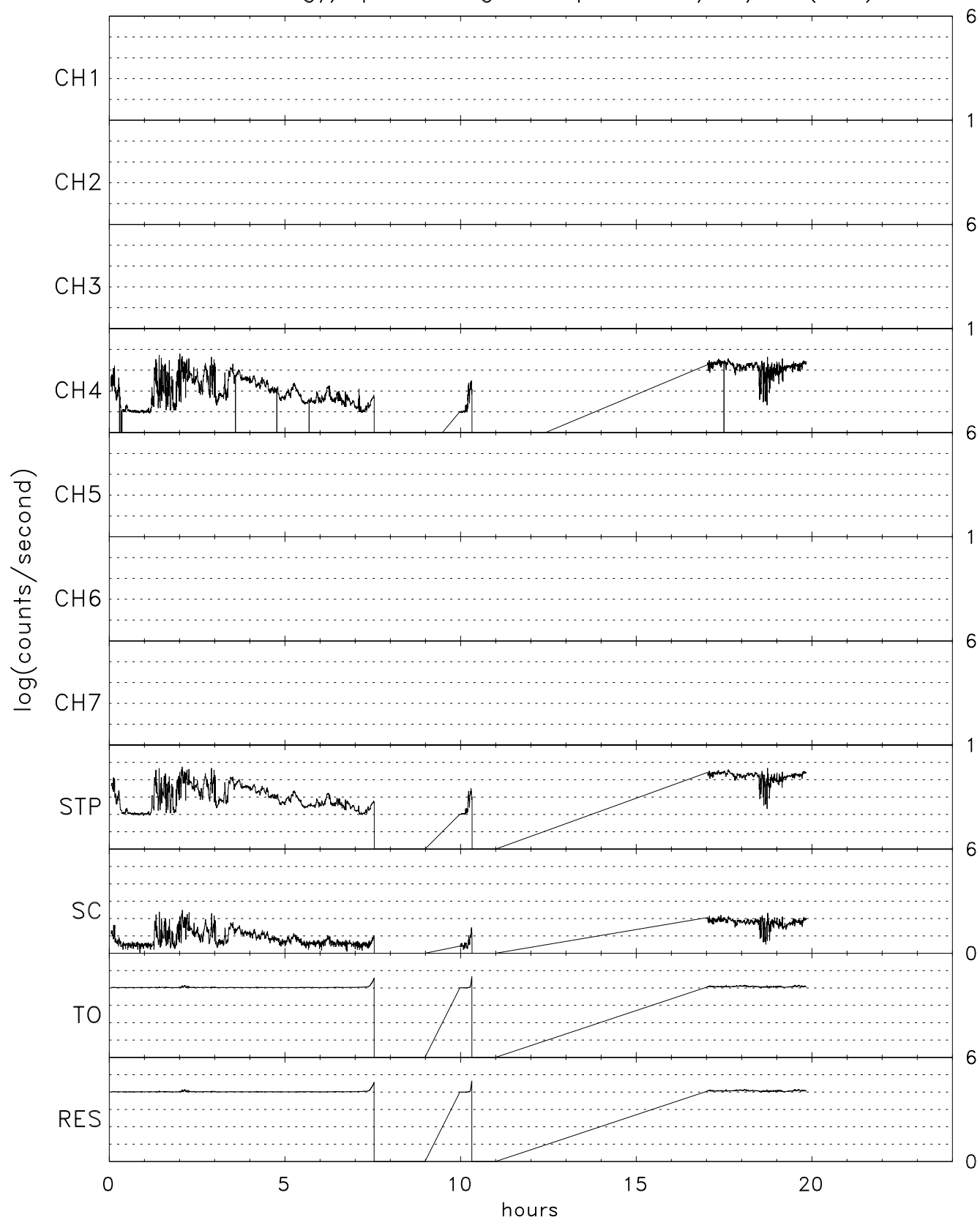
TIDE energy/spin averaged Stops for 12/27/07 (361)
