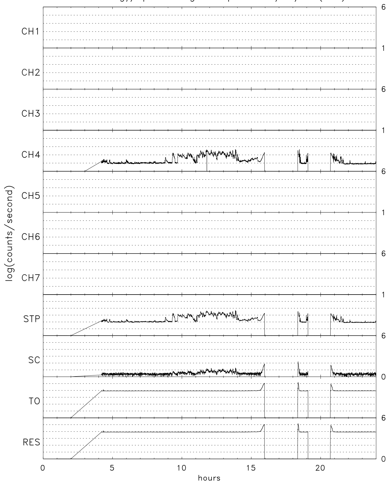
TIDE energy/spin averaged Stops for 12/22/07 (356)
