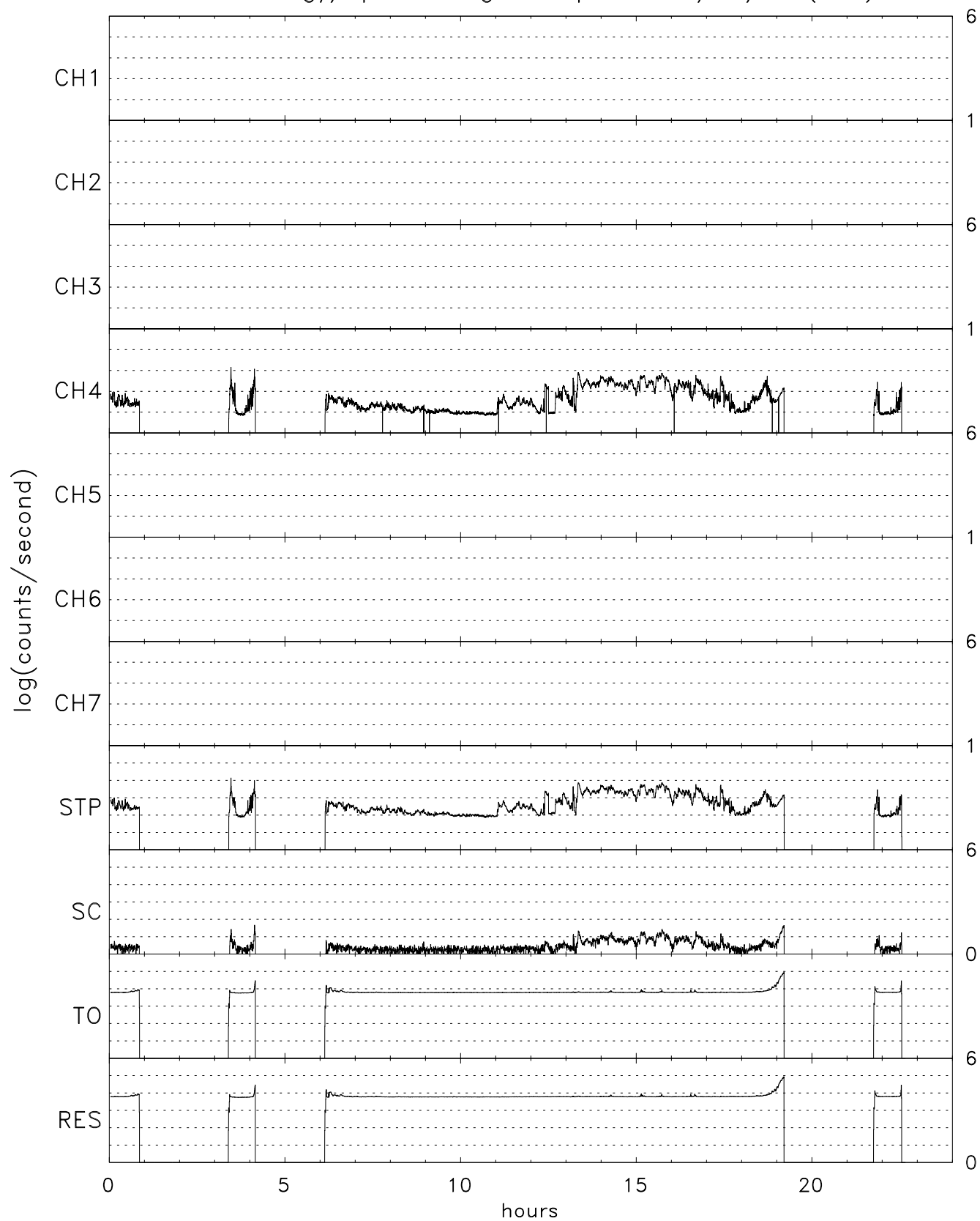
TIDE energy/spin averaged Stops for 12/18/07 (352)
