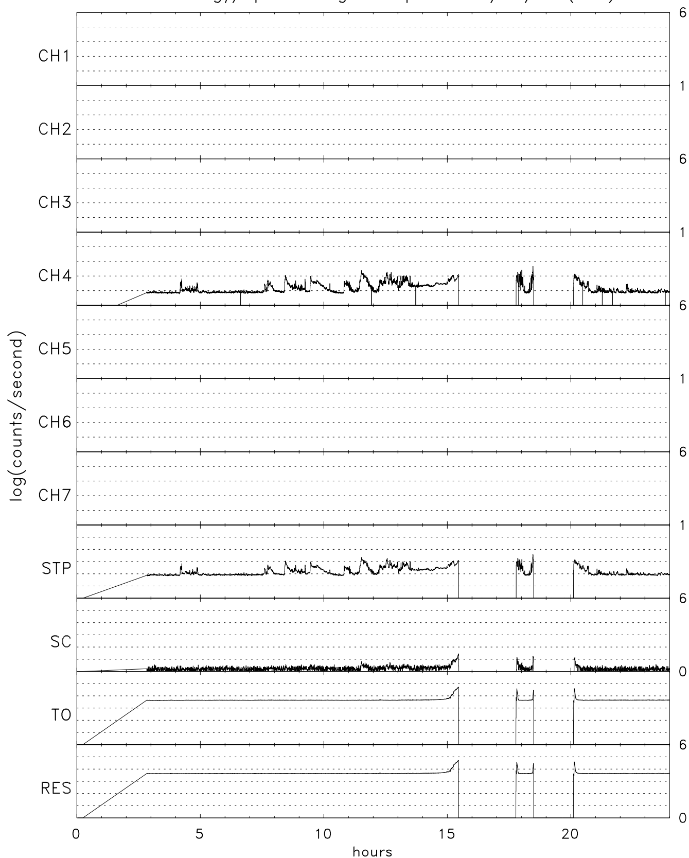
TIDE energy/spin averaged Stops for 12/12/07 (346)
