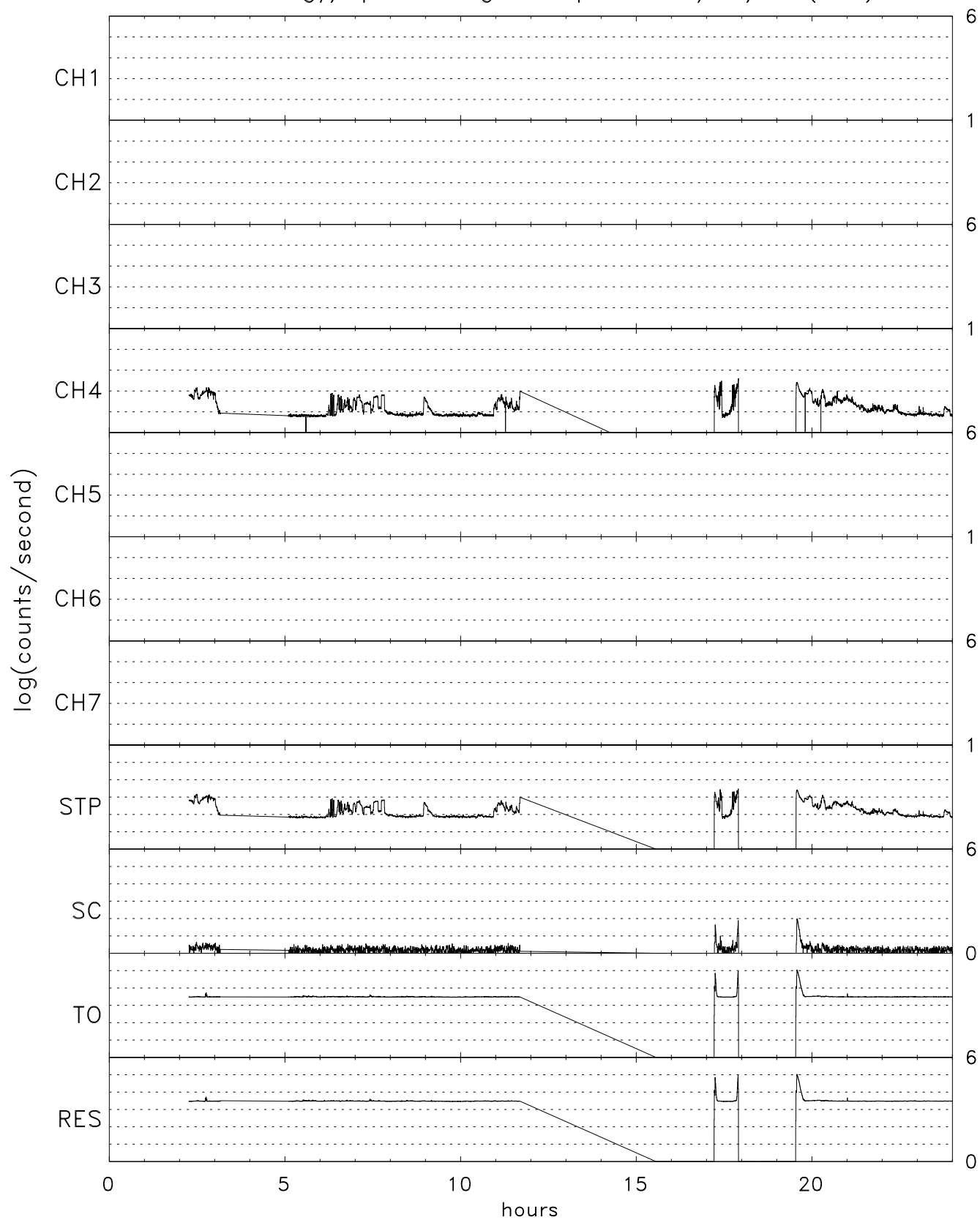
TIDE energy/spin averaged Stops for 12/02/07 (336)
