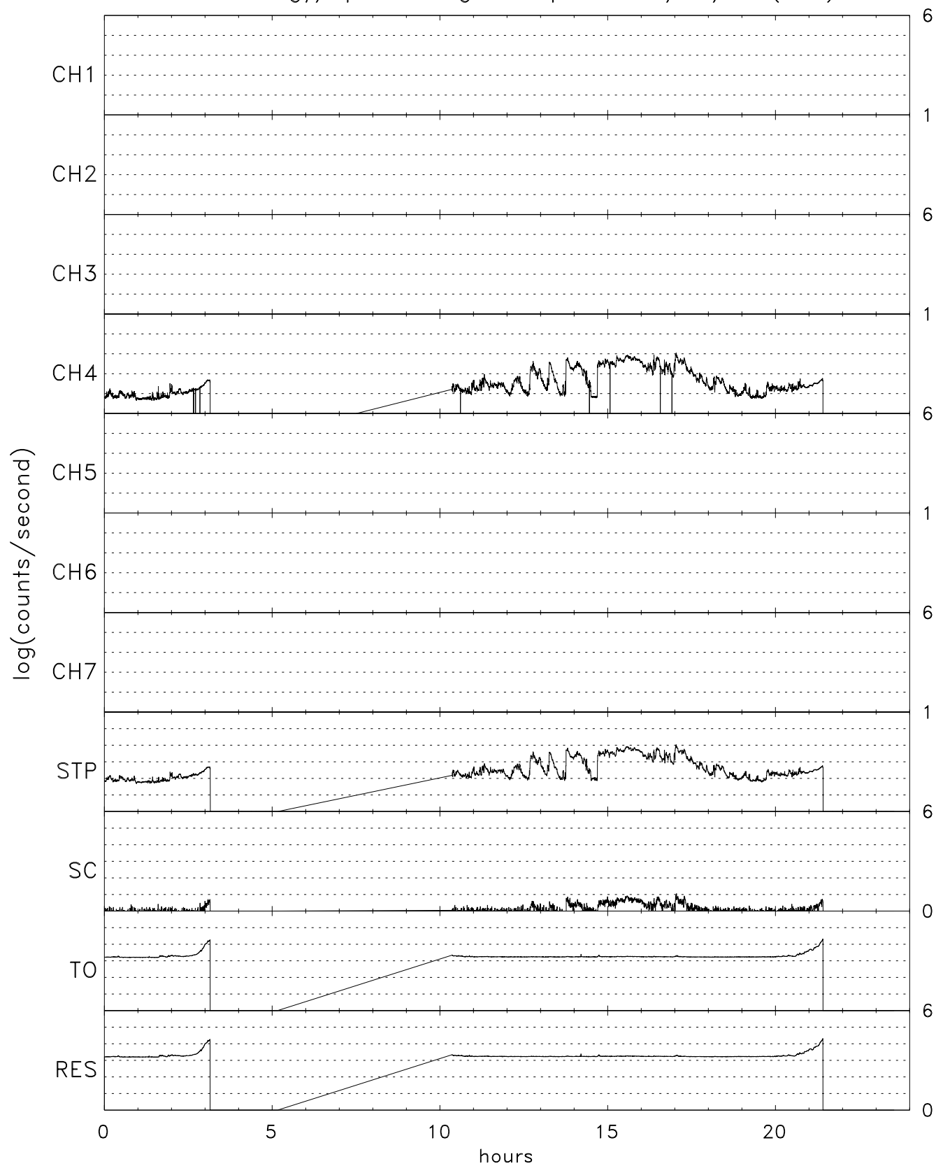
TIDE energy/spin averaged Stops for 11/24/07 (328)
