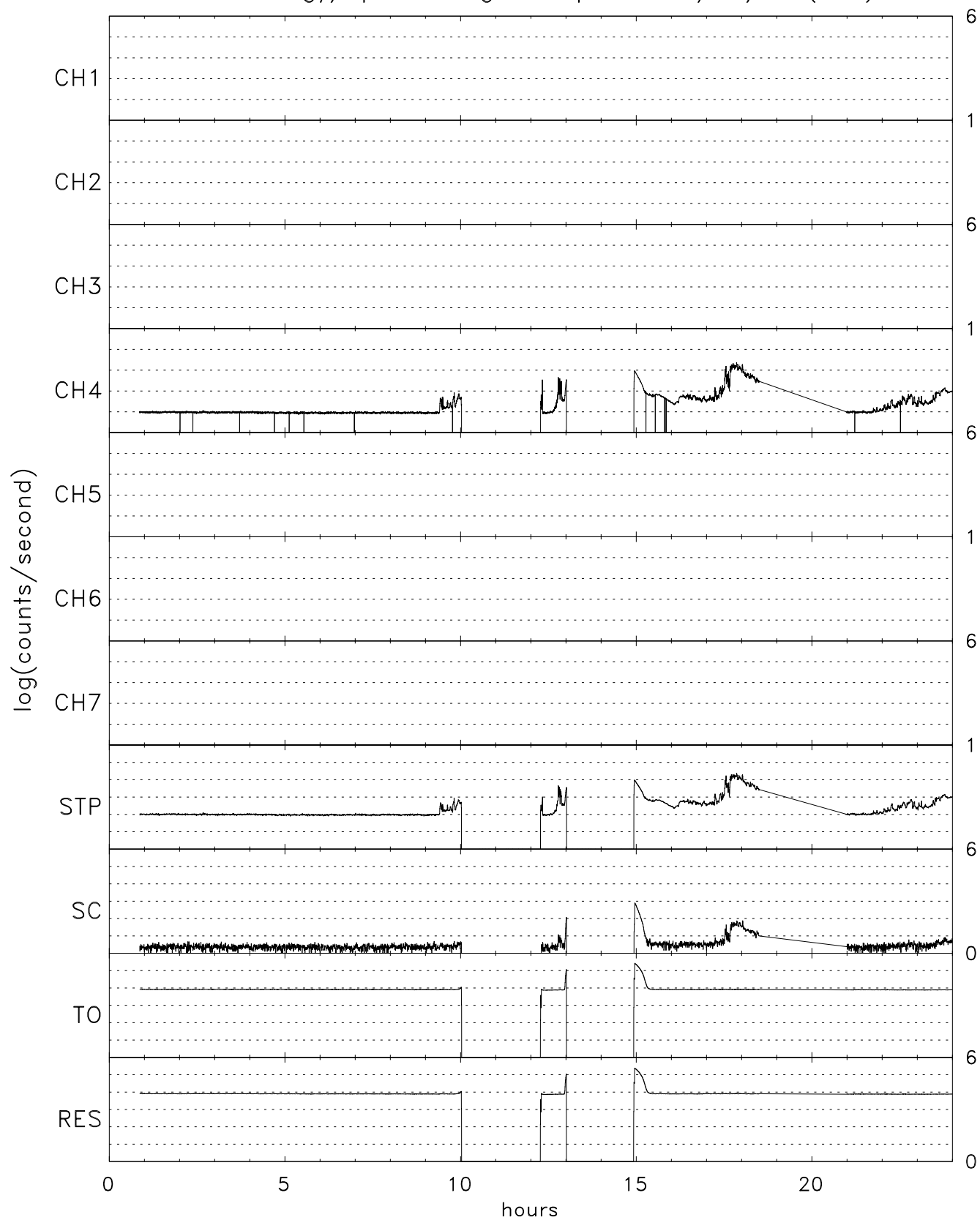
TIDE energy/spin averaged Stops for 10/10/07 (283)
