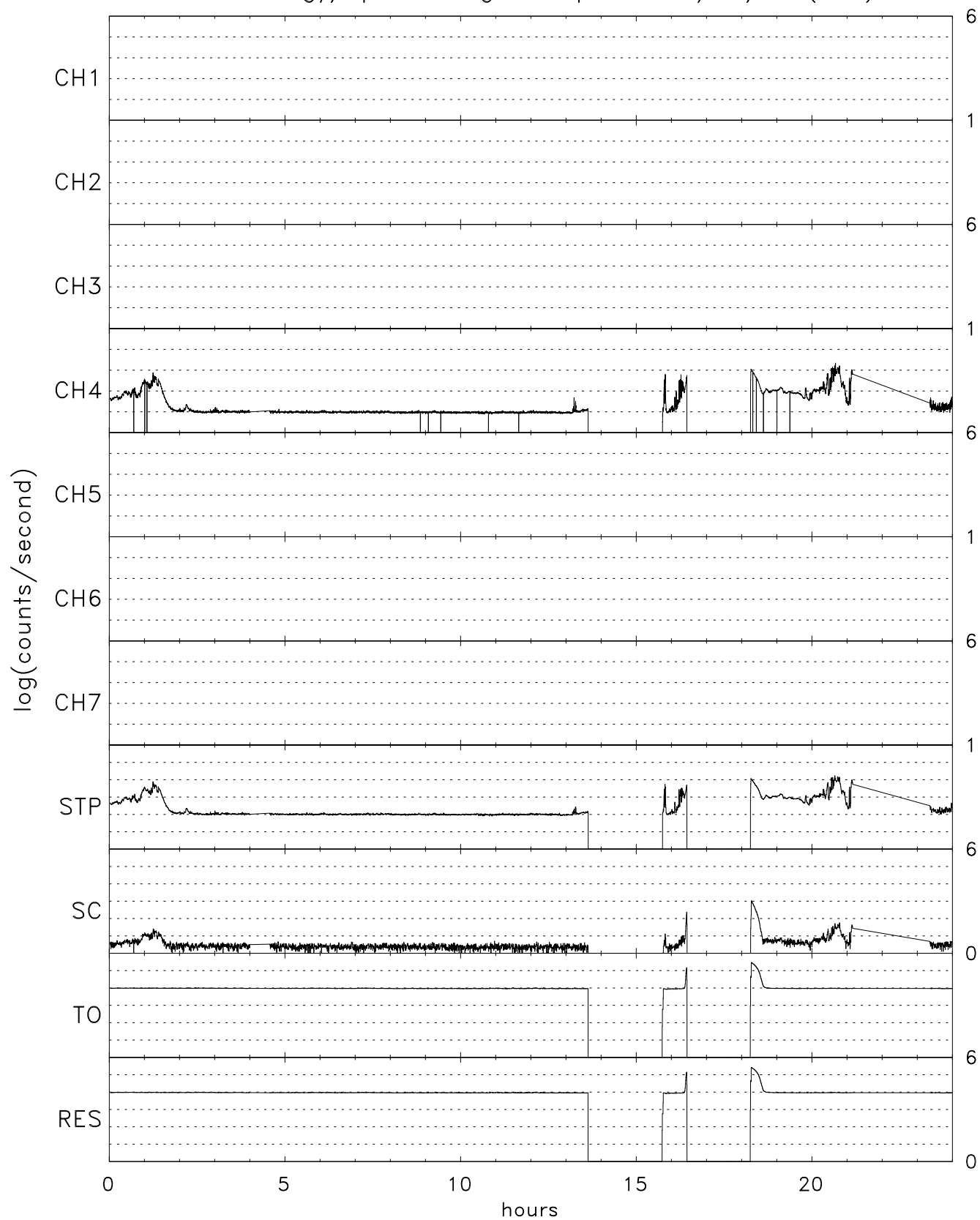
TIDE energy/spin averaged Stops for 10/06/07 (279)
