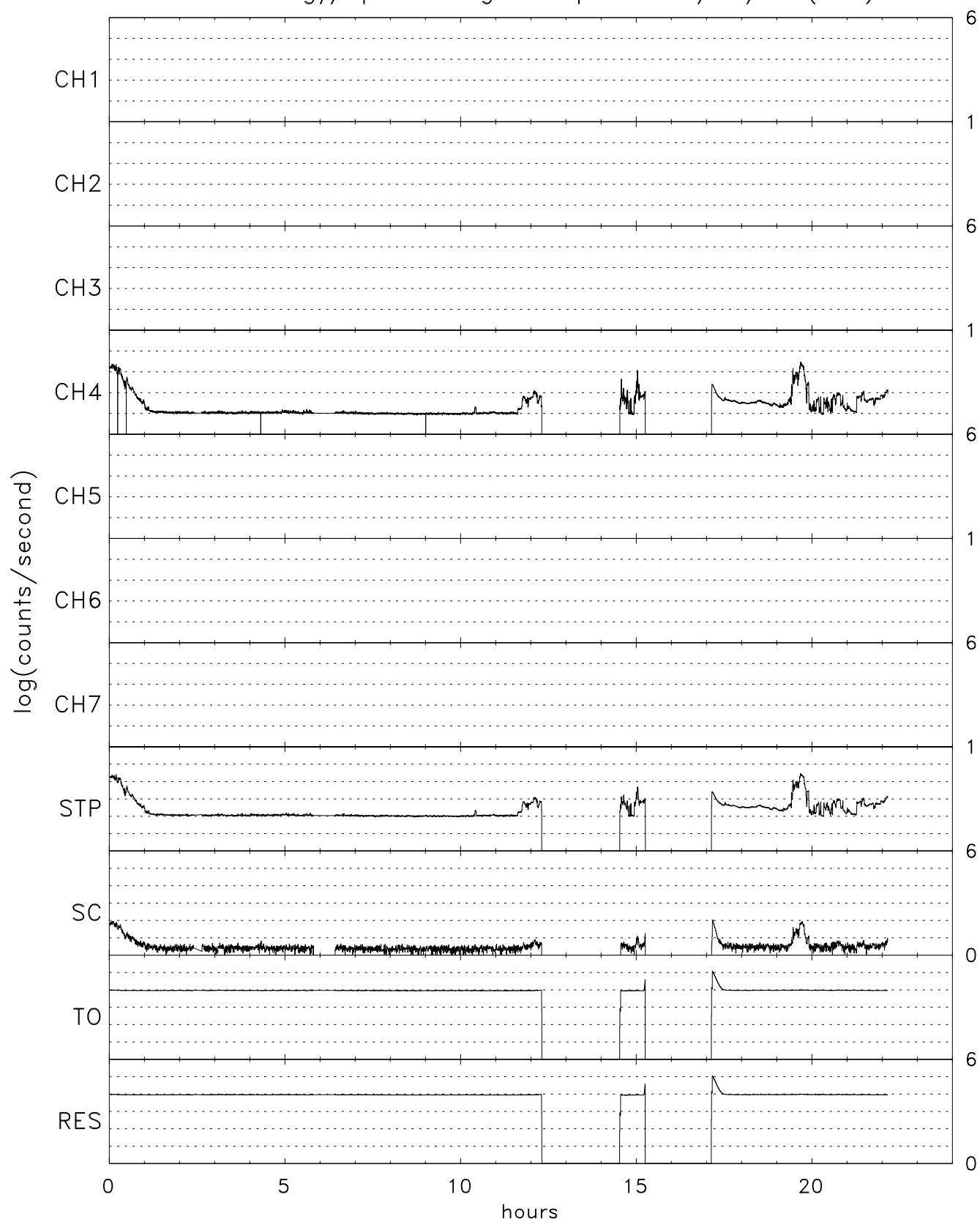
TIDE energy/spin averaged Stops for 09/16/07 (259)
