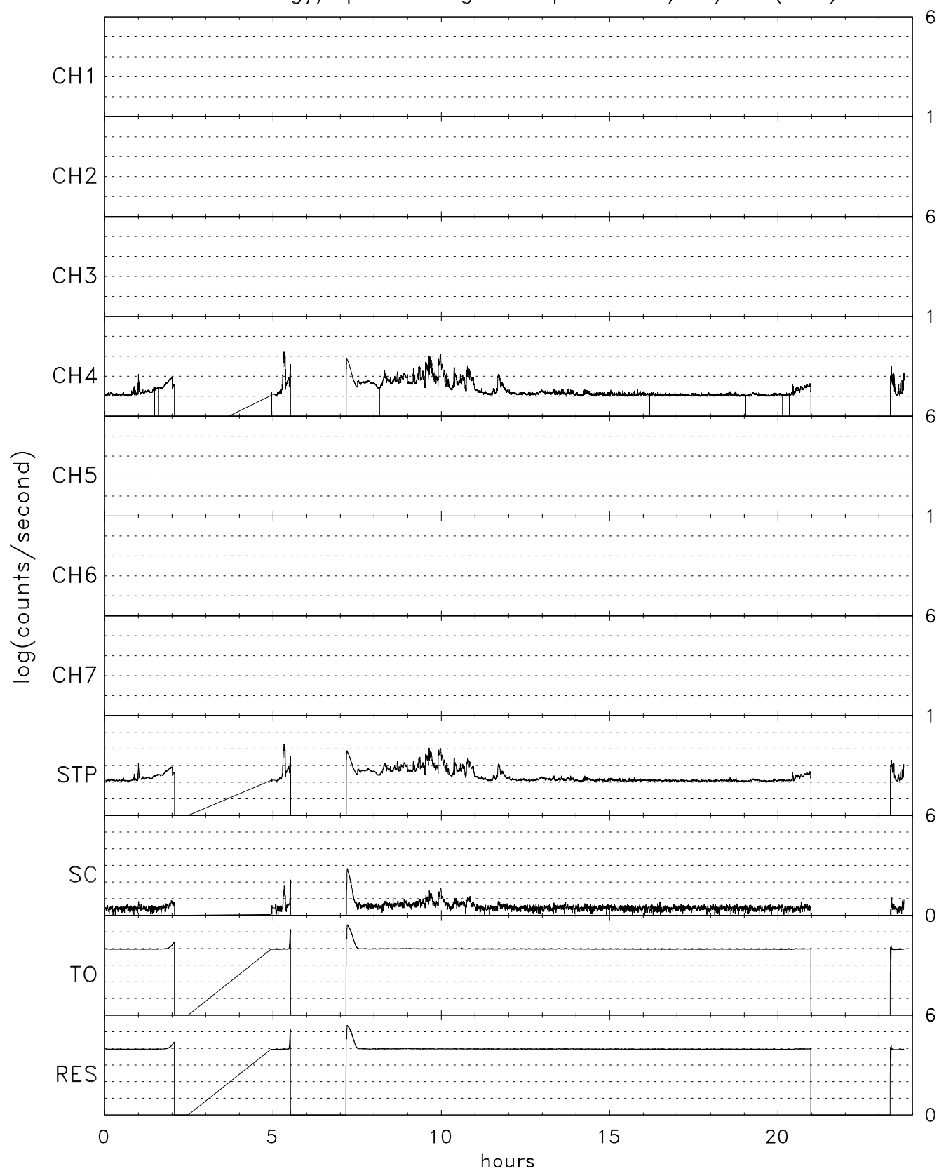
TIDE energy/spin averaged Stops for 09/11/07 (254)
