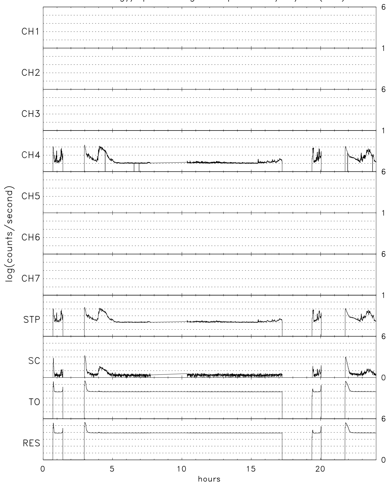
TIDE energy/spin averaged Stops for 09/05/07 (248)
