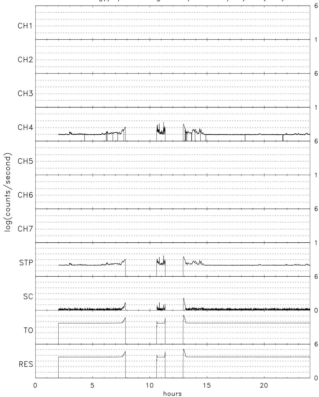
TIDE energy/spin averaged Stops for 06/19/07 (170)
