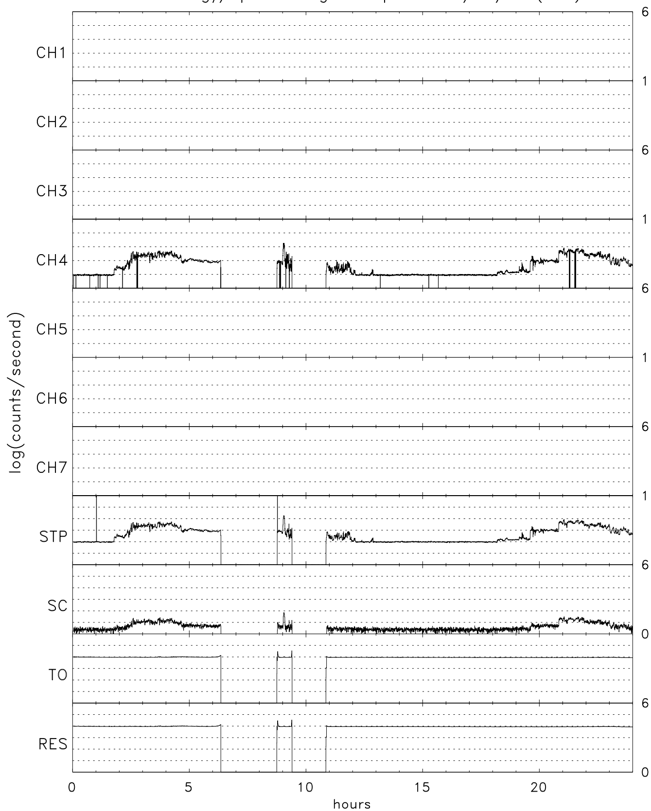
TIDE energy/spin averaged Stops for 04/11/07 (101)
