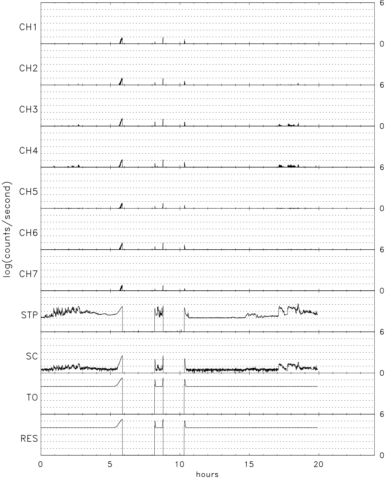
TIDE energy/spin averaged 0+ for 03/19/07 (078)
