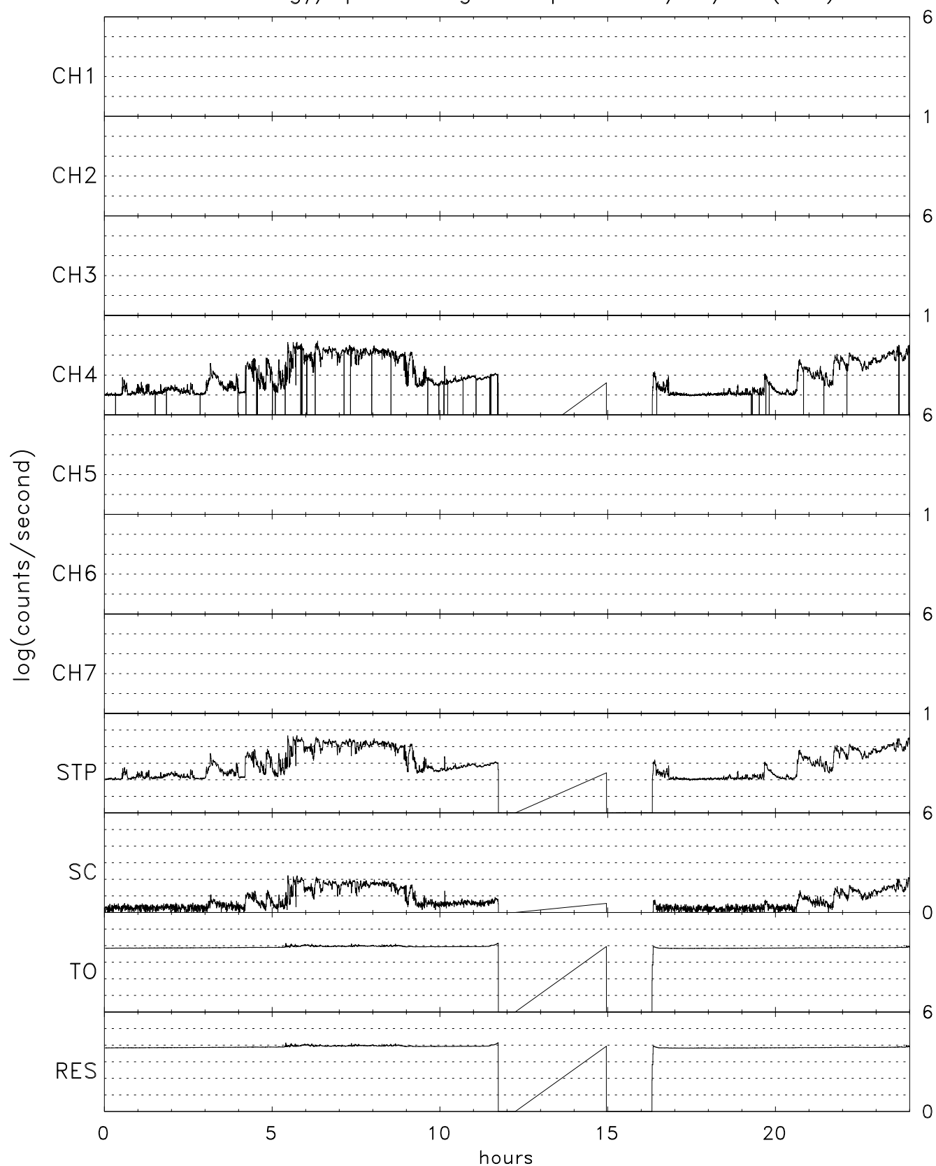
TIDE energy/spin averaged Stops for 02/13/07 (044)
