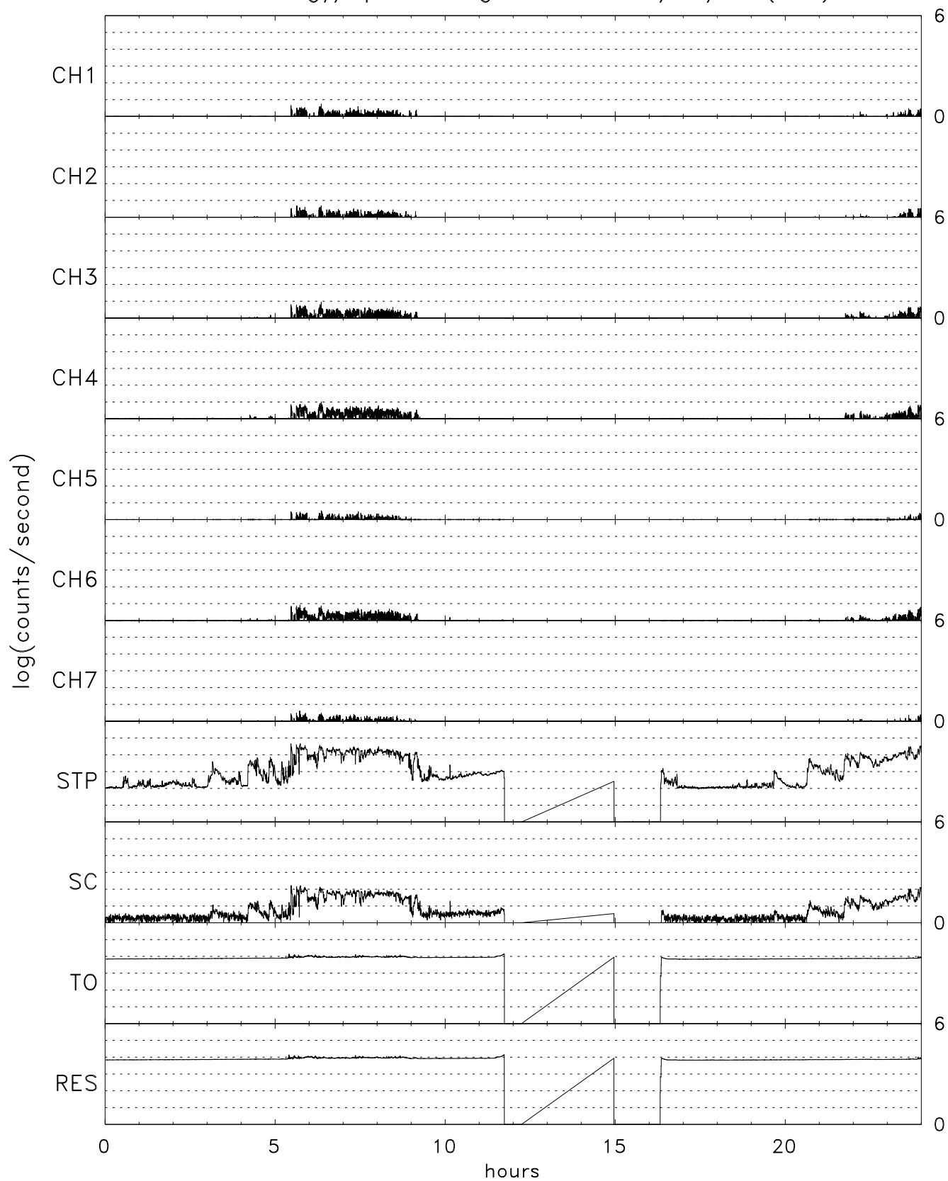
TIDE energy/spin averaged 0+ for 02/13/07 (044)
