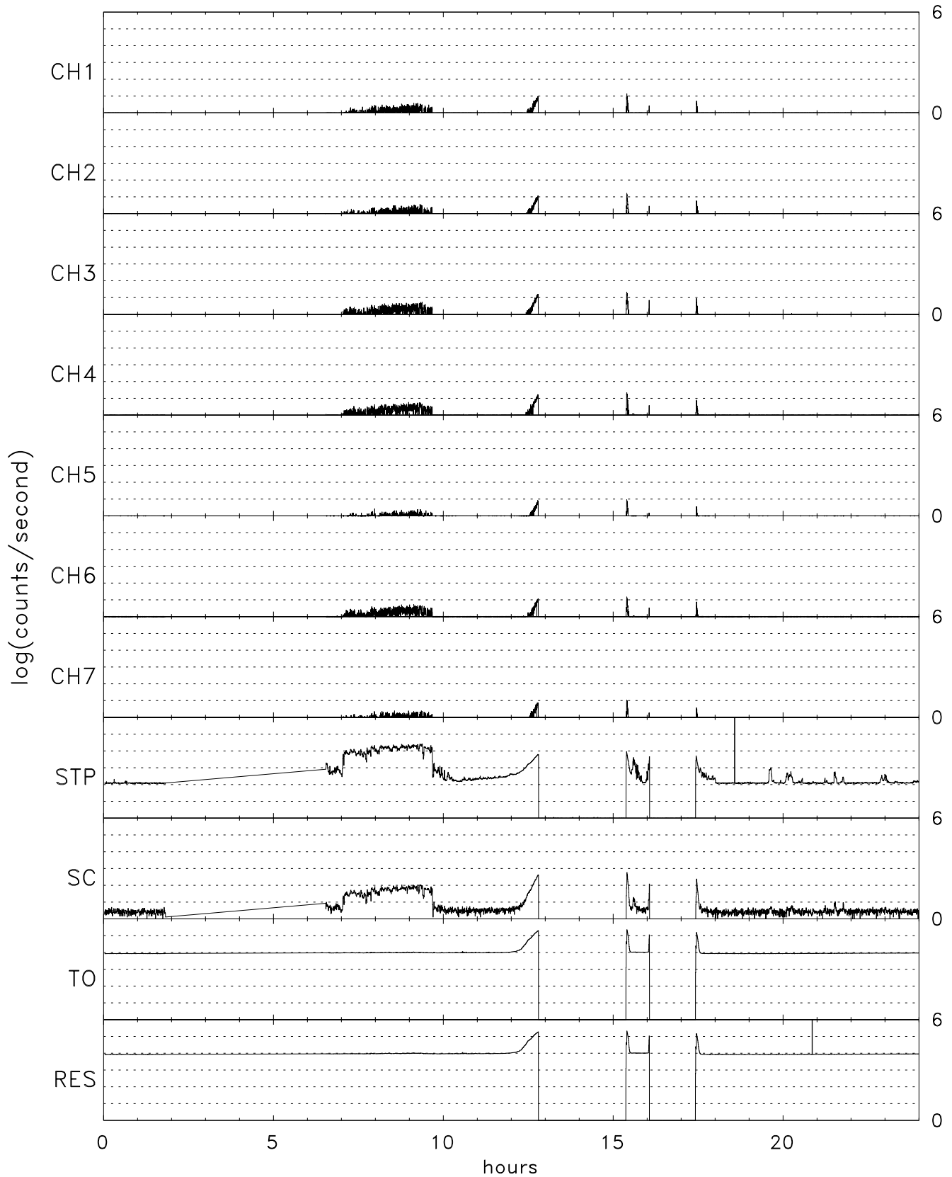
TIDE energy/spin averaged 0+ for 02/03/07 (034)
