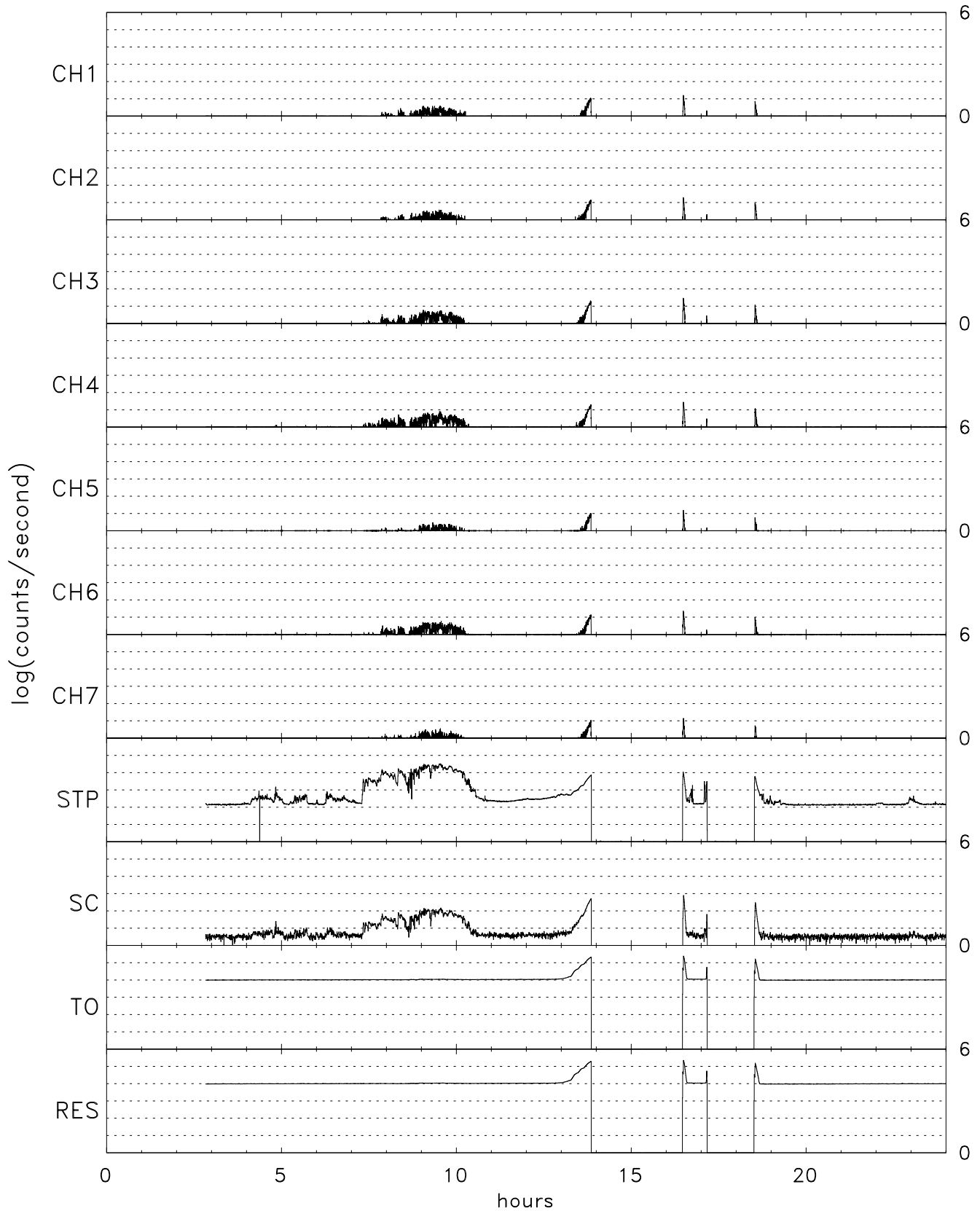
TIDE energy/spin averaged 0+ for 01/24/07 (024)
