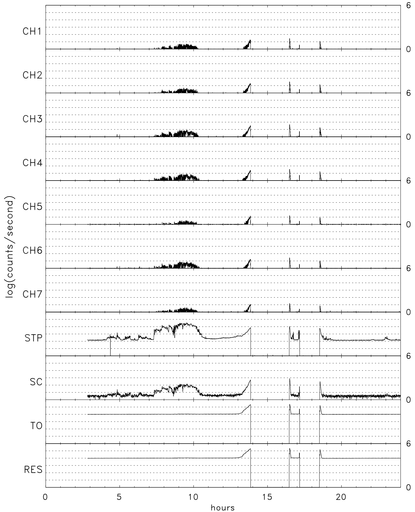
TIDE energy/spin averaged H+ for 01/24/07 (024)
